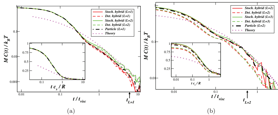
FIG. 6. Normalized VACF C(t)/(k_B T/M) for a neutrally buoyant hard spherical bead of mass M suspended in a fluid of I -DSMC particles of diameter D , for two different bead sizes, a small bead of radius R = 1.25D (a) and a large bead of radius R = 6.25D (b). A log-log scale is used to emphasize the long-time power law tail, and the time is normalized by the viscous time t_{visc} , so that the results should be approximately independent of the actual bead radius. The inset shows the initial decay of the VACF on a semi-log scale, where the time is normalized by the sonic time scale t_c . Periodic boundary conditions with a cubic cell of length L are employed, and the sound crossing time t_L is indicated. Results from purely particle simulations are shown with a dashed-dotted line, and the incompressible hydrodynamic theory is shown in with a dotted line. Results from hybrid runs are also shown with a solid line for the stochastic hybrid and dashed line for the deterministic hybrid, for both the same box size as the particle runs (red) and a larger simulation box (green).
