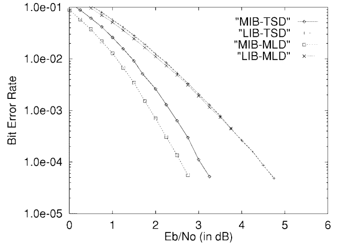
Fig. 2. Error performance of code S3: MLD and TSD of the MIB's and LIB's.
