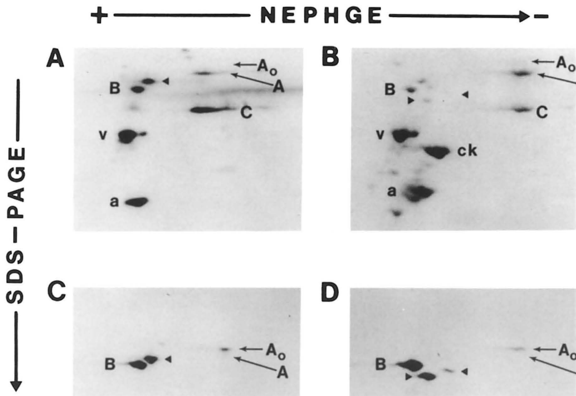
Figure 1. Identification of R-[2- 14 C]mevalonate-labeled proteins in CHO-K1 and HeLa nuclear lamina-intermediate filament preparations by 2D-NEPHGE and fluorography. CHO-K1 and HeLa cells were labeled with 2 \mu Ci/ml R-(2- 14 C) mevalonate for 17 h in medium IV. Nuclear lamina intermediate filament fractions were analyzed by 2D-NEPHGE and fluorography as previously described (4). Proteins were visualized by silver staining. (A) Silver-stained CHO-K1 nuclear lamina intermediate filament preparation. (B) Silver-stained HeLa nuclear lamina intermediate filament preparation. (C and D) Fluorograms of the 2D-NEPHGE gels in A and B, respectively. Only the relevant portion of each fluorogram is shown. Fluorographic exposure was for 45 d. Indicated are lamins A (72 kD), B (68 kD), and C (62 kD); the 74-kD isoprenylated prelamin A polypeptide ( A o ), the 70-kD lamina-associated isoprenylated polypeptide ( solid triangle ), vimentin ( v ), and actin ( a ). The arrows in A and B (as well as in subsequent figures) indicate the relative position of prelamin A ( A o ) and lamin A in C and D as determined by superimposing each fluorogram on its silver-stained gel.
