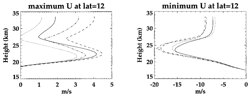
FIG. 15. As in Fig. 14, except for the zonal wind at 12^\circ latitude.
