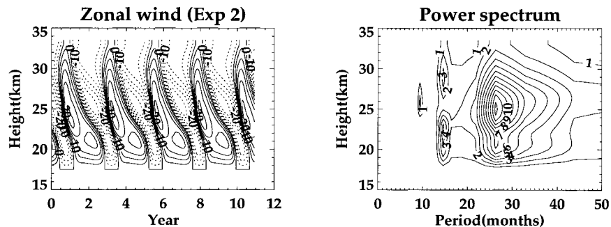
FIG. 13. As in Fig. 3, except for expt 2.
