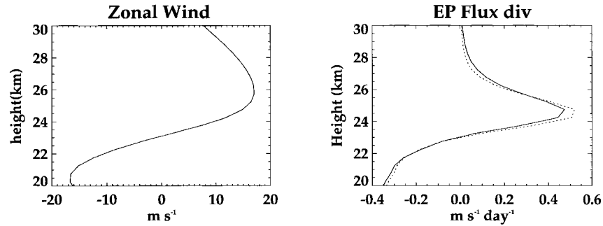
FIG. 12. (a) Zonal wind at the equator on day 1900 in \text{m s}^{-1} . (b) Vertical profile of the latitudinally integrated density weighted EP flux divergence ( \text{m s}^{-1} \text{day}^{-1} ), calculated using the basic-state profile from day 1900. The solid lines denote calculations made from the RS, and the dashed lines denote calculations made from expt 1.
