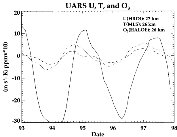
FIG. 10. Time series of the equatorial observed zonal wind (from UARS HRDI), and anomalies (observed value minus time mean) of temperature (from UARS MLS) and ozone volume mixing ratio (from UARS HALOE) near 26-km altitude. Zonal wind is given in \text{m s}^{-1} (solid line), temperature in K (dotted line), and ozone mixing ratio in \text{ppmv} \times 10 (dashed line).
