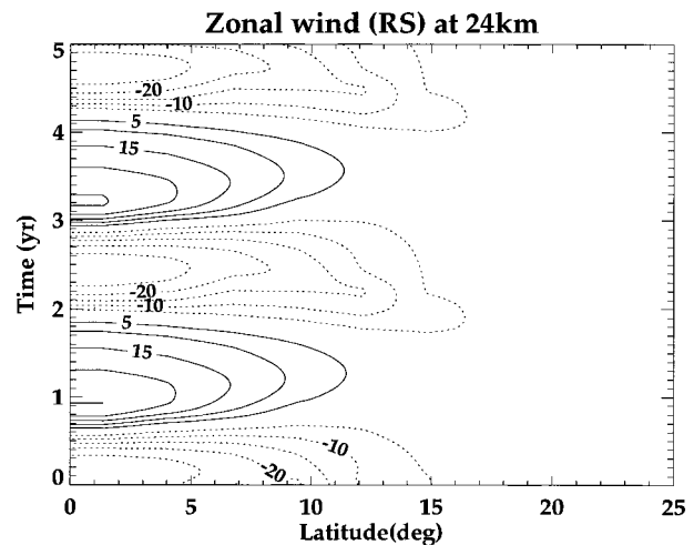
FIG. 5. Latitude–time cross section of the zonal wind at 24 km. Contour interval is 5 m s ^{-1} , and dotted contours represent easterly winds.
