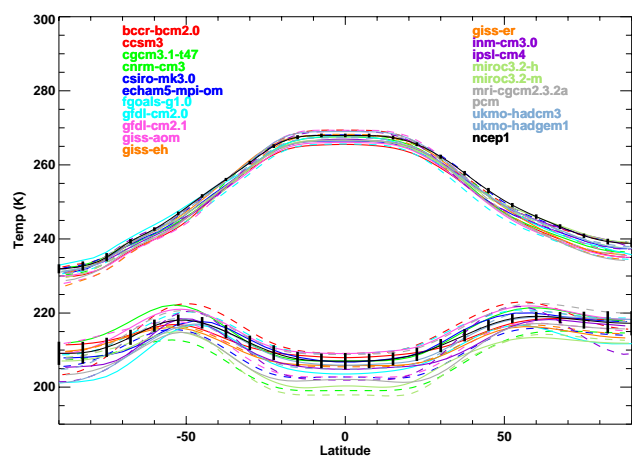
Fig. 3. Zonally and annually averaged temperature at 500 hPa (upper) and 50 hPa (lower) between 1979–1999 from the climate models and NCEP. The 2\text{-}\sigma variation in the NCEP reanalysis is shown in the heavy black vertical lines, and the colors are as in Fig. 2.
