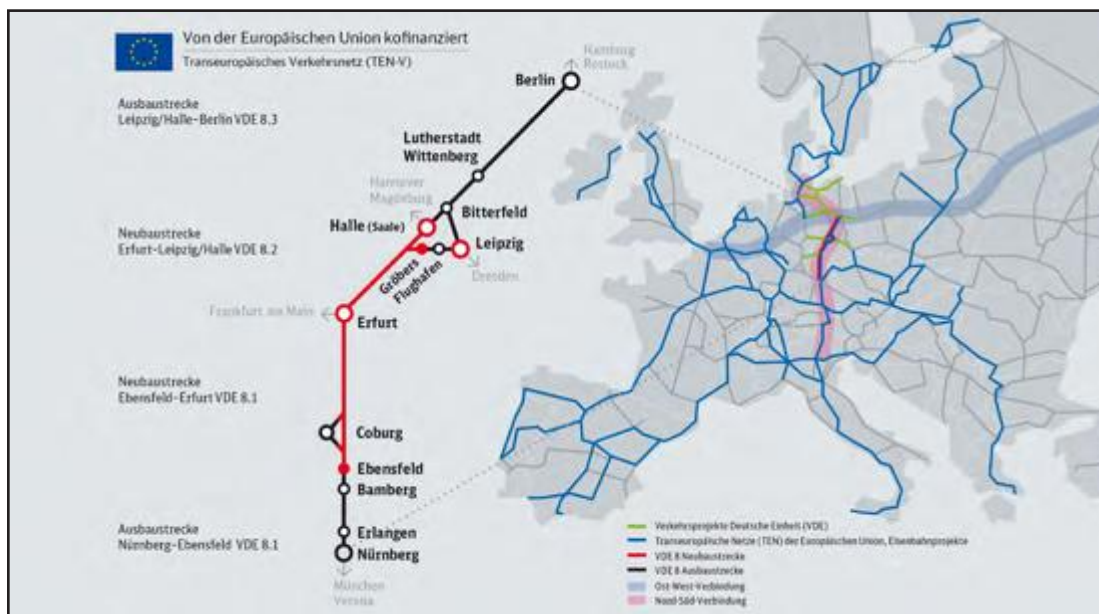
Figure 50. The Leipzig and Erfurt Nodes within the Context of VDE8 and TEN-T1
