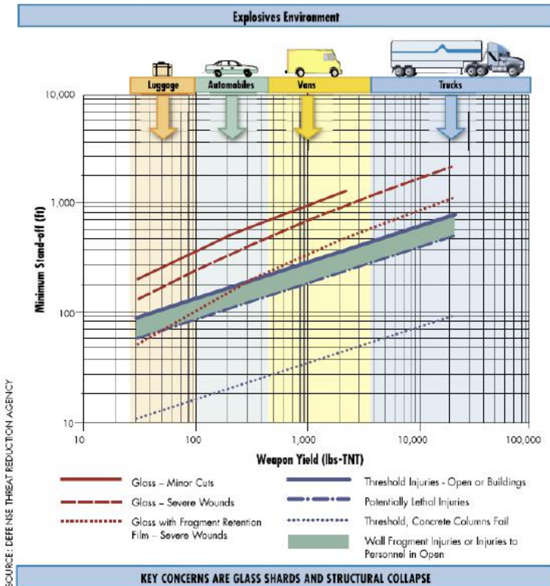
Figure 2 Distances of Concern for Explosive Overpressure
