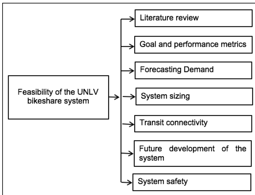
Figure 2. Research Framework
