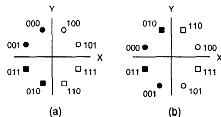
Fig. 1: (a) Non-standard and (b) hybrid labelings of an 8-PSK constellation.
