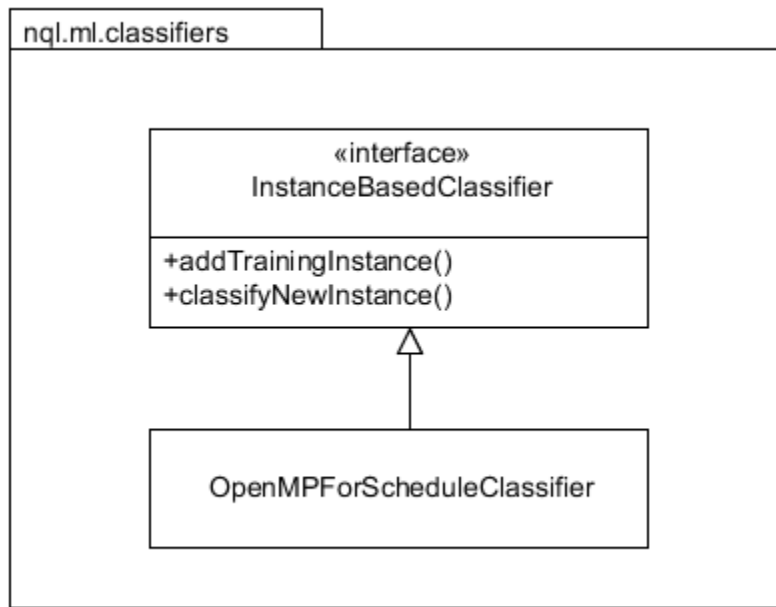
Figure 41. Classes Under nql.ml.classifiers Package
