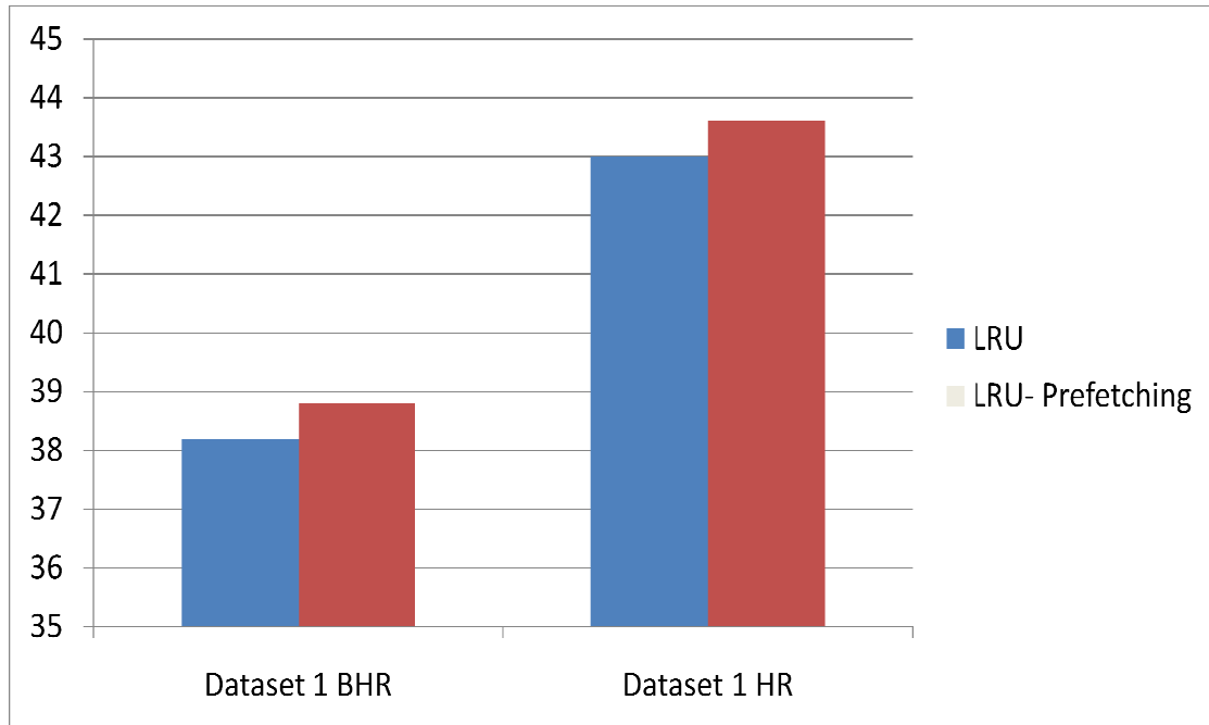
Figure 12: Dataset 1: LRU Vs Pre-fetching based LRU
