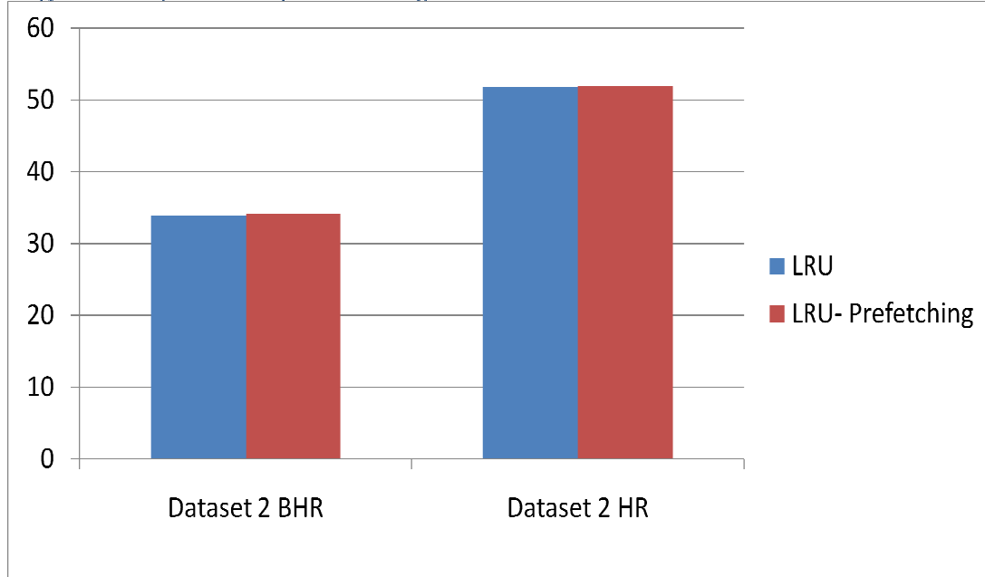
Figure 14: Dataset 2: LRU Vs Pre-fetching based LRU
