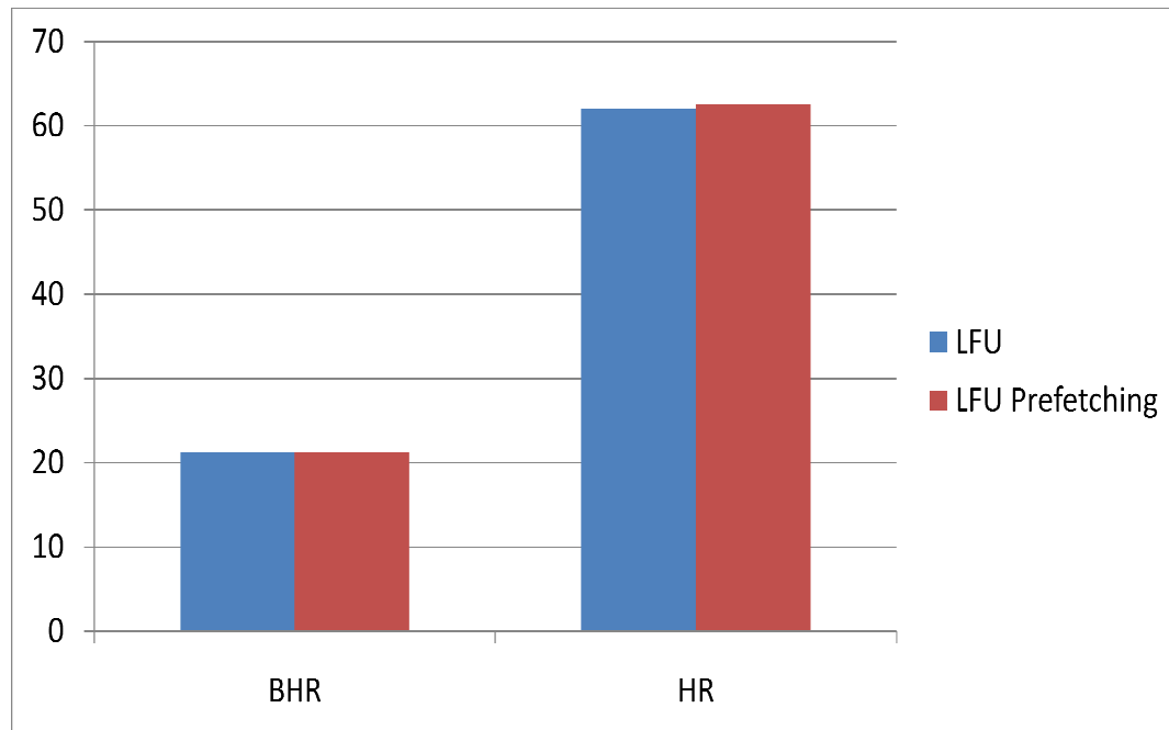
Figure 19: Dataset 4: LFU Vs Pre-fetching based LFU
