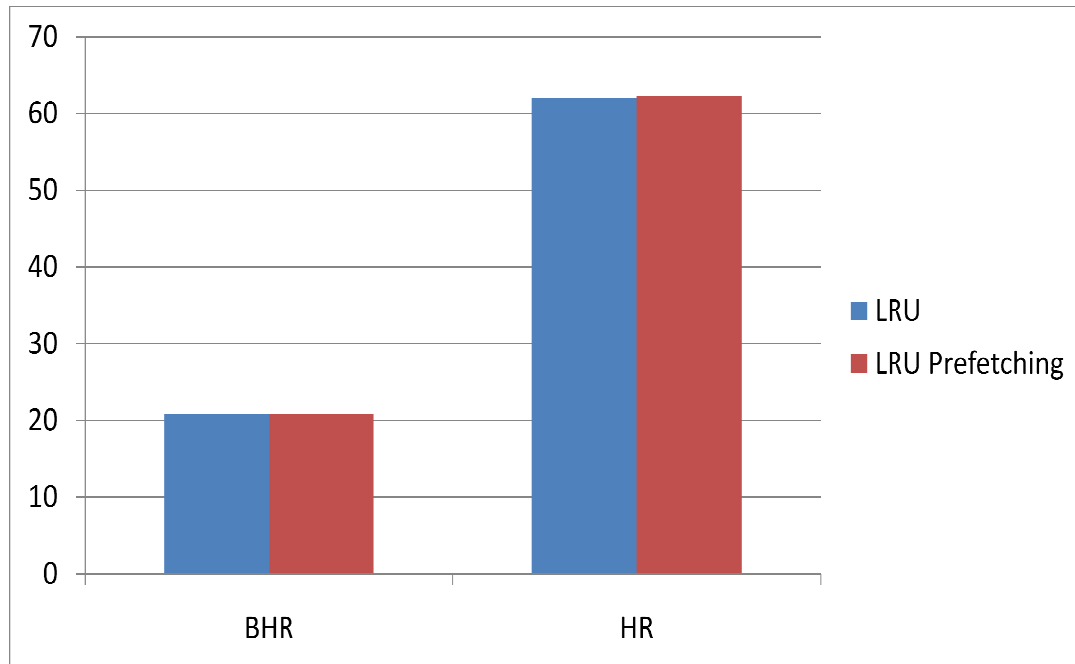
Figure 18: Dataset 4 LRU Vs Pre-fetching based LRU
