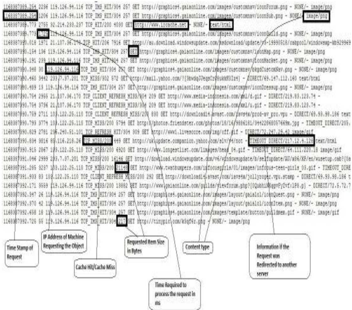
Figure 1: Snapshot of an Actual Proxy Server Log File
