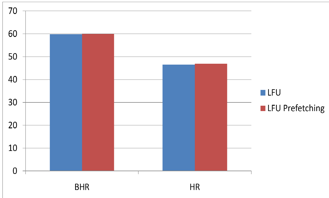
Figure 17: Dataset 3 LFU Vs Pre-fetching based LFU
