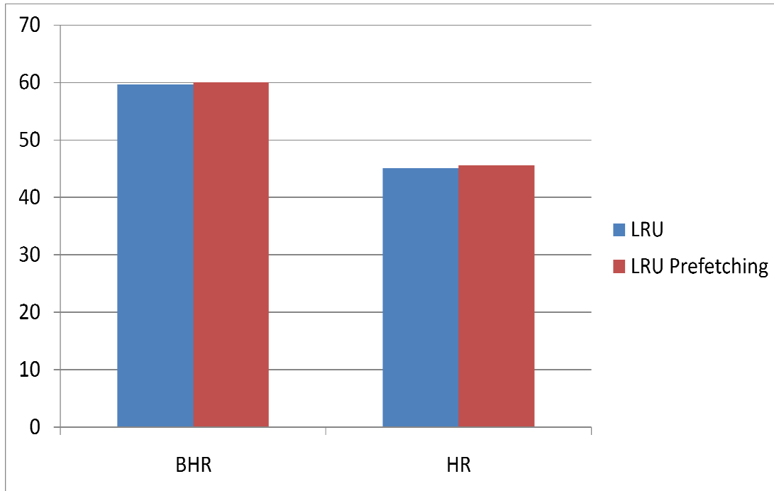
Figure 16: Dataset 3: LRU Vs Pre-fetching based LRU
