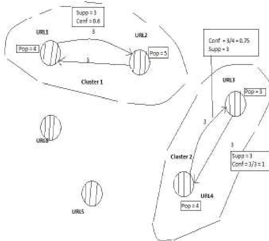
Figure 9: Graph after using the Breadth First Search
