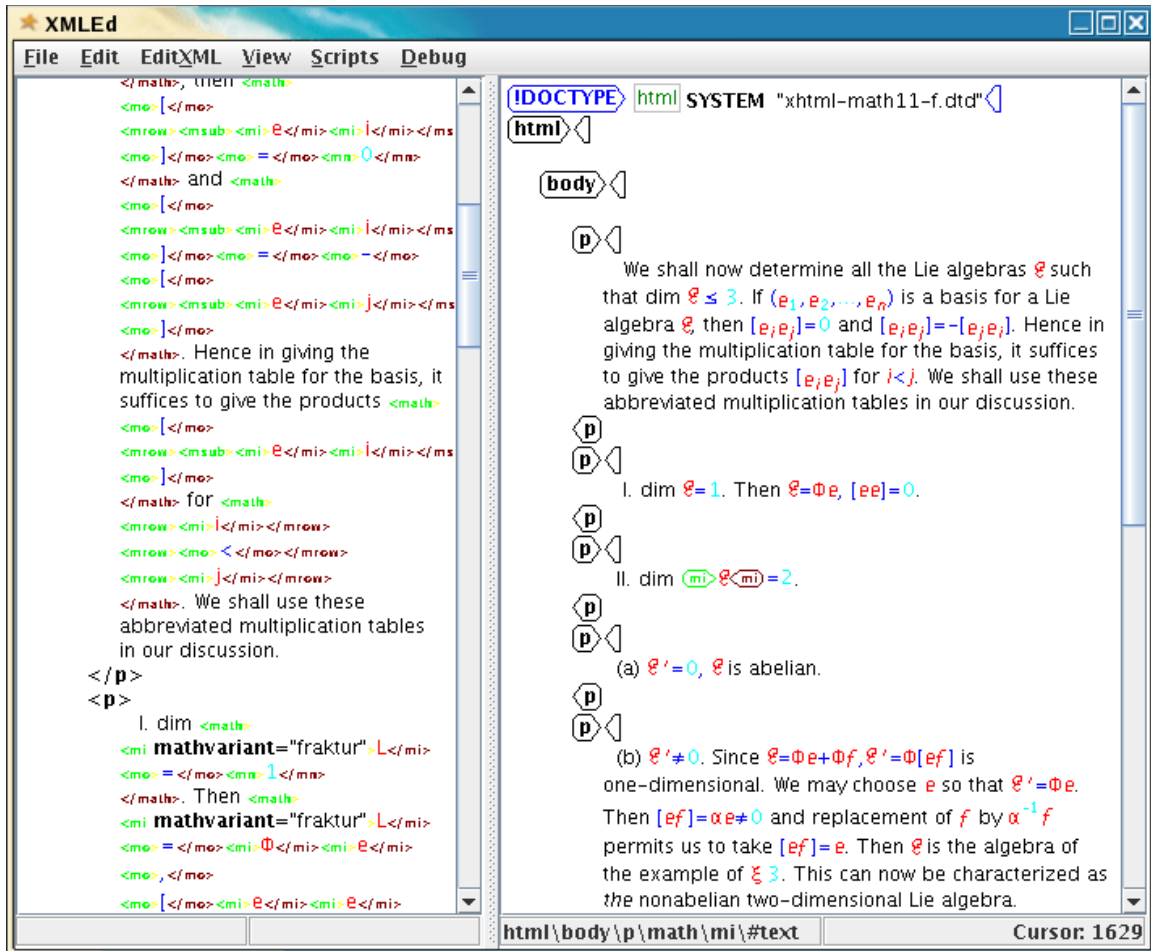
Illustration 6.16.: Zoom Mode Tag Level 0
