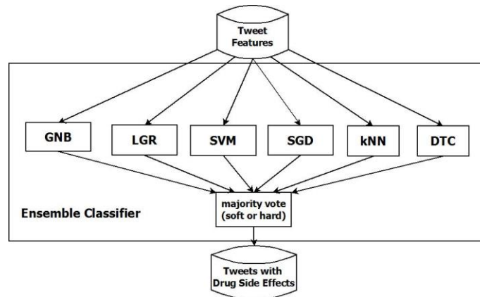
Figure 2: Ensemble Classifier with 6 classifiers and a soft or hard majority vote of the classifier predictions
