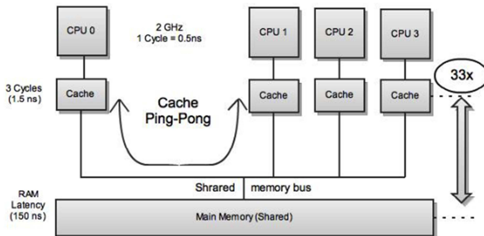
Figure 25 Cache Ping-ponging on multi-level memory in a multiprocessor system
