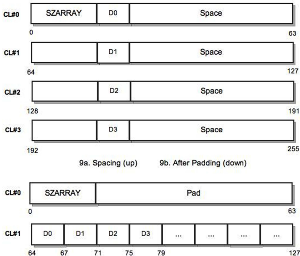
Figure 9. Cache line structure with Spacing only and Padding only techniques
