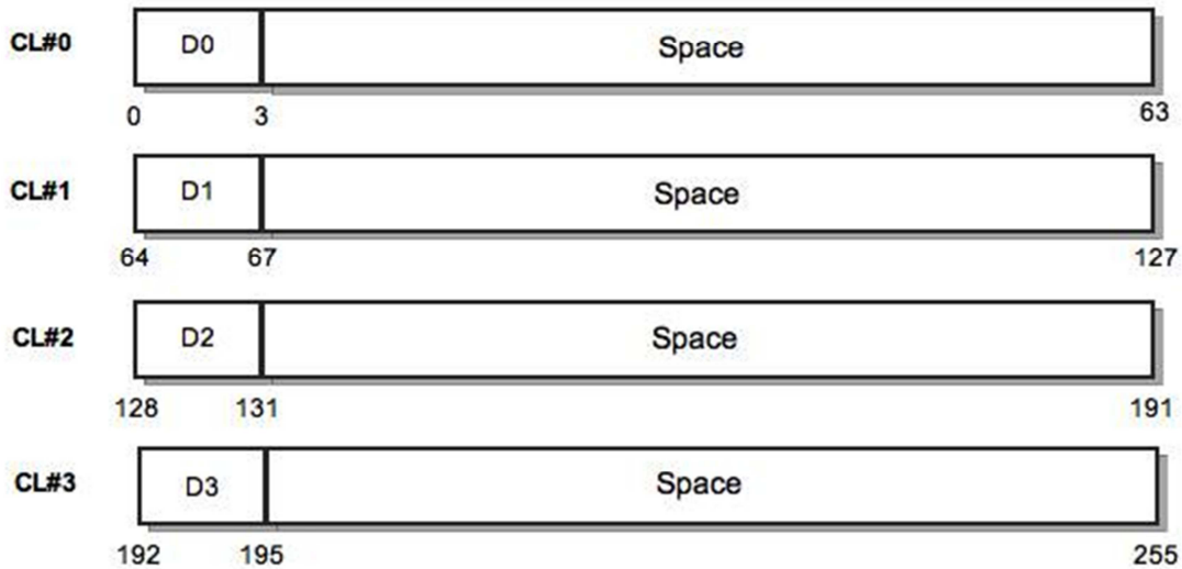
Figure 8. Cache line structure with Spacing technique
