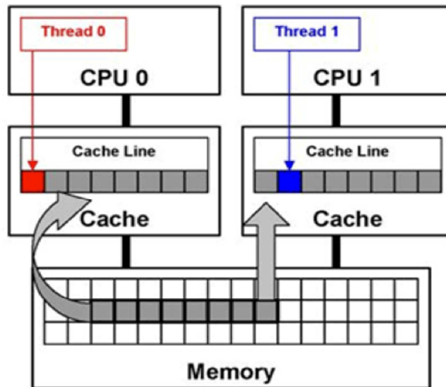
Figure 4. False cache line sharing on SMP [7]
