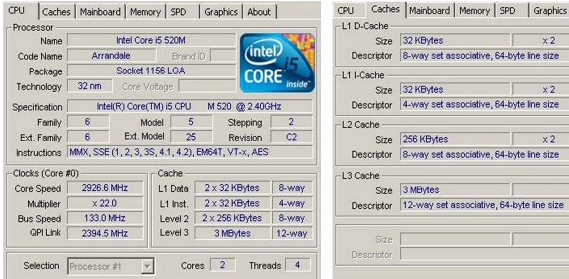
Figure 14. Intel Core i5 520M CPU and cache specifications [13]
