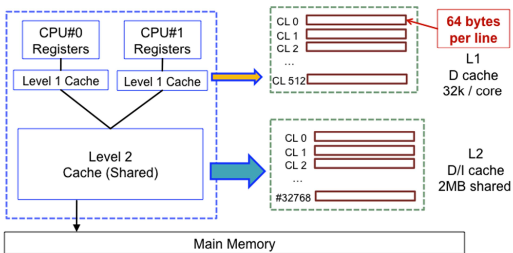
Figure 3. Cache line details of Intel Core2 T5270 processor [2]
