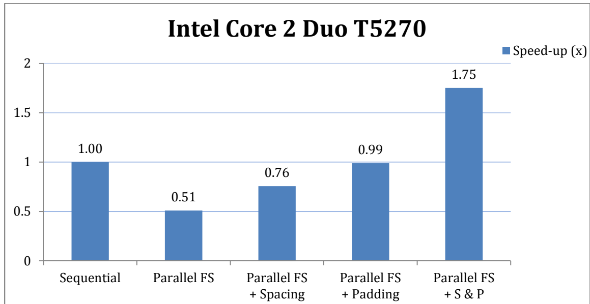
Figure 17. Speed-up ratios on Intel Core2 Duo T5270 test system
