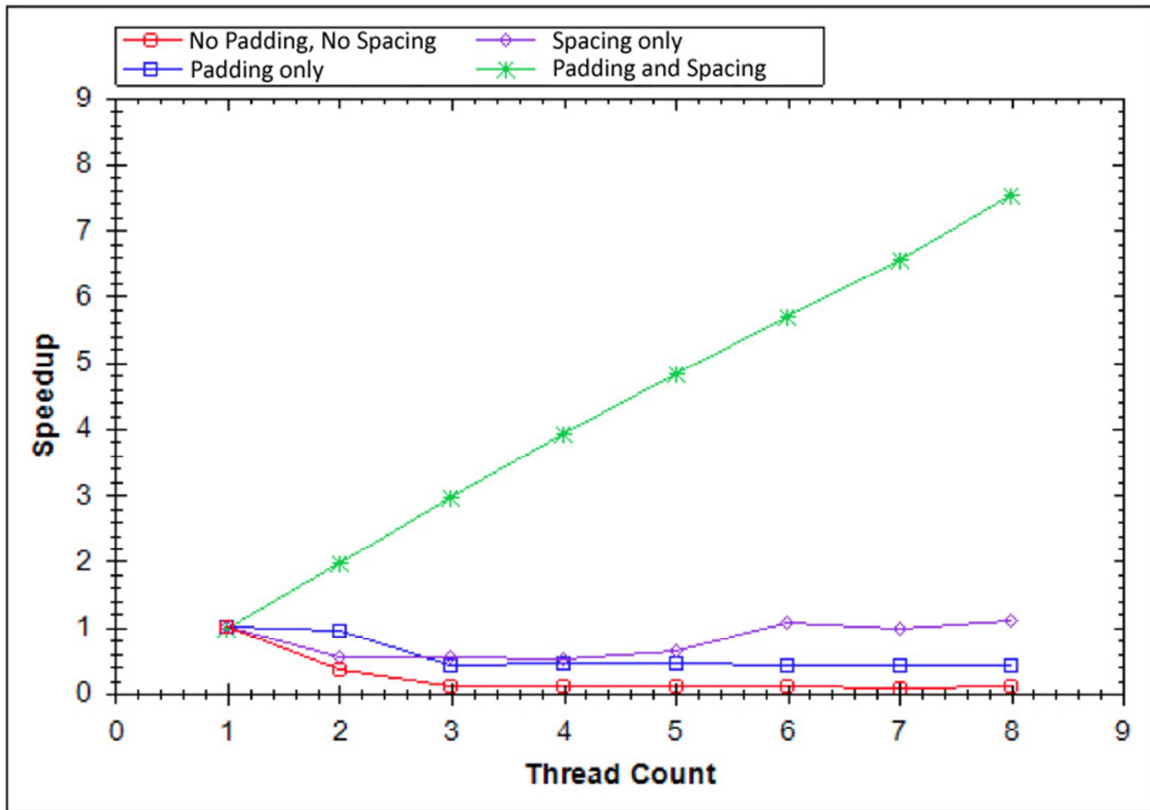
Figure 6. Speed-up results from Padding and Spacing employed on testing array [8]
