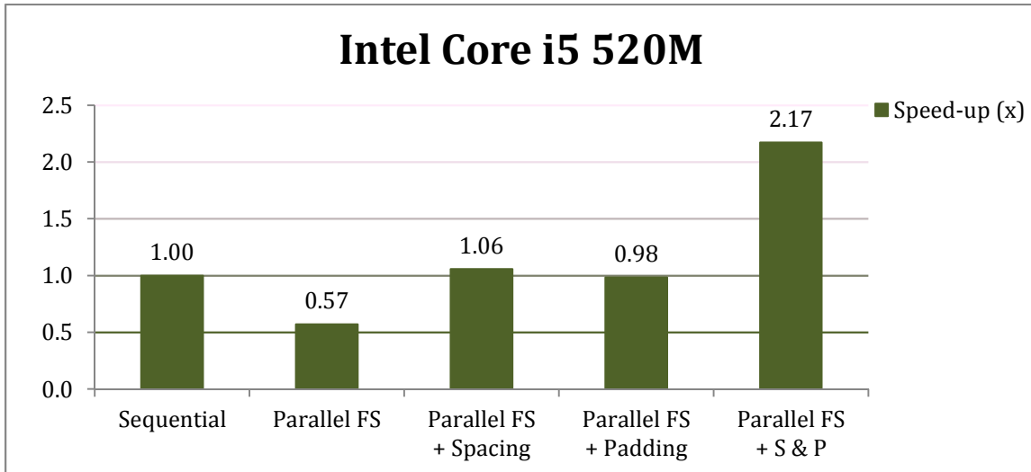
Figure 23. Speed-up ratios on Intel Core i5 520M test system
