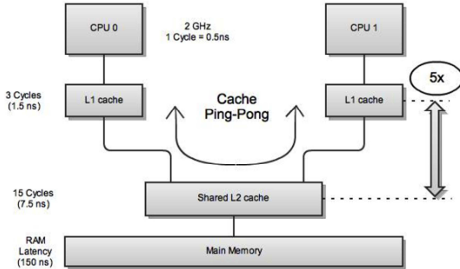
Figure 26. Cache Ping-ponging on multi-level memory in a dual core system
