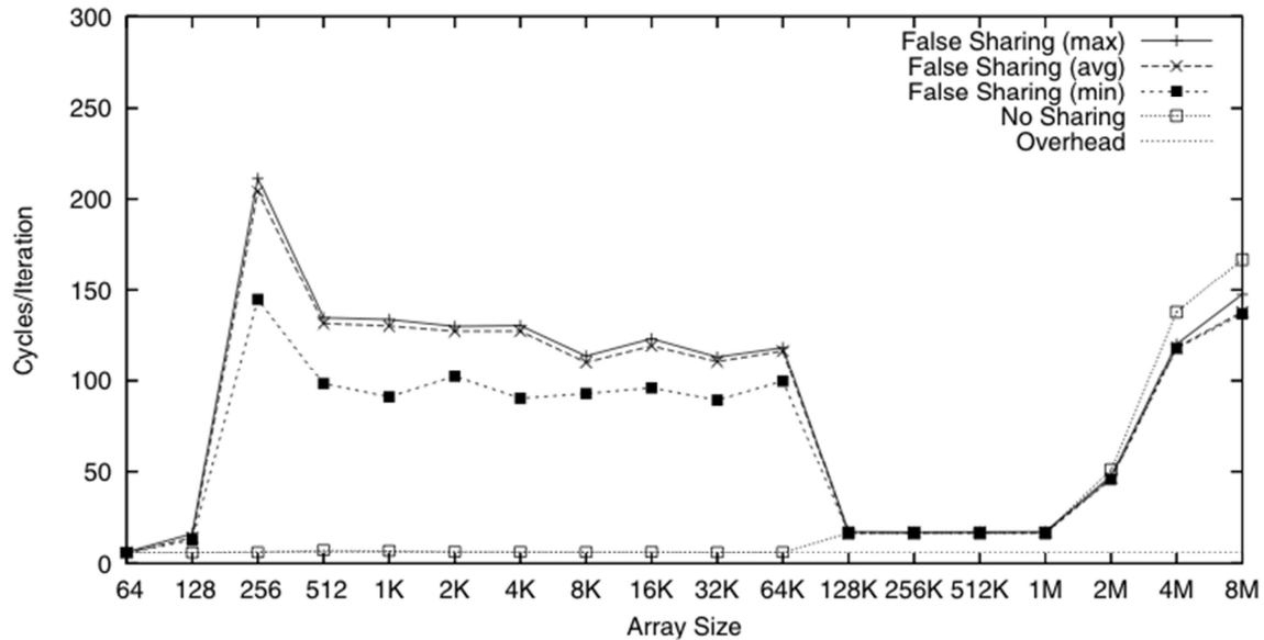
Figure 7. Number of latency cycles on varied array size, Intel Core Duo 2600 [16]
