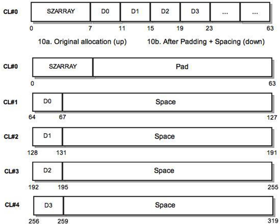
Figure 10. Cache line structure with combined Padding and Spacing technique
