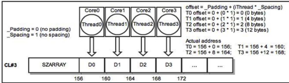
11a. Cache line structure of Parallel FS case (up)
