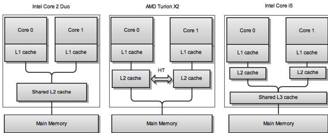
Figure 2. Memory hierarchy in CMP [5]
