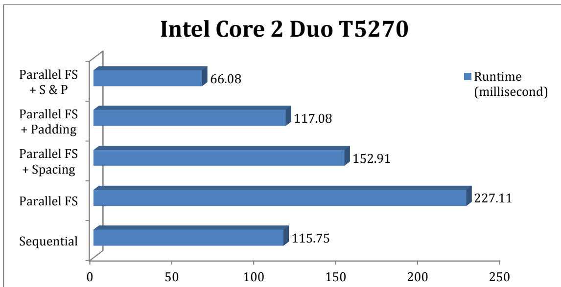
Figure 16. Average runtime on Intel Core2 Duo T5270 test system
