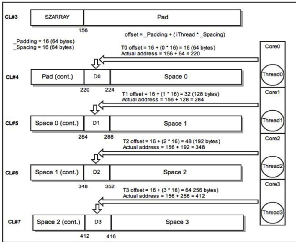
11b. Cache line Structure of Parallel FS + Padding + Spacing remedies case (down)
