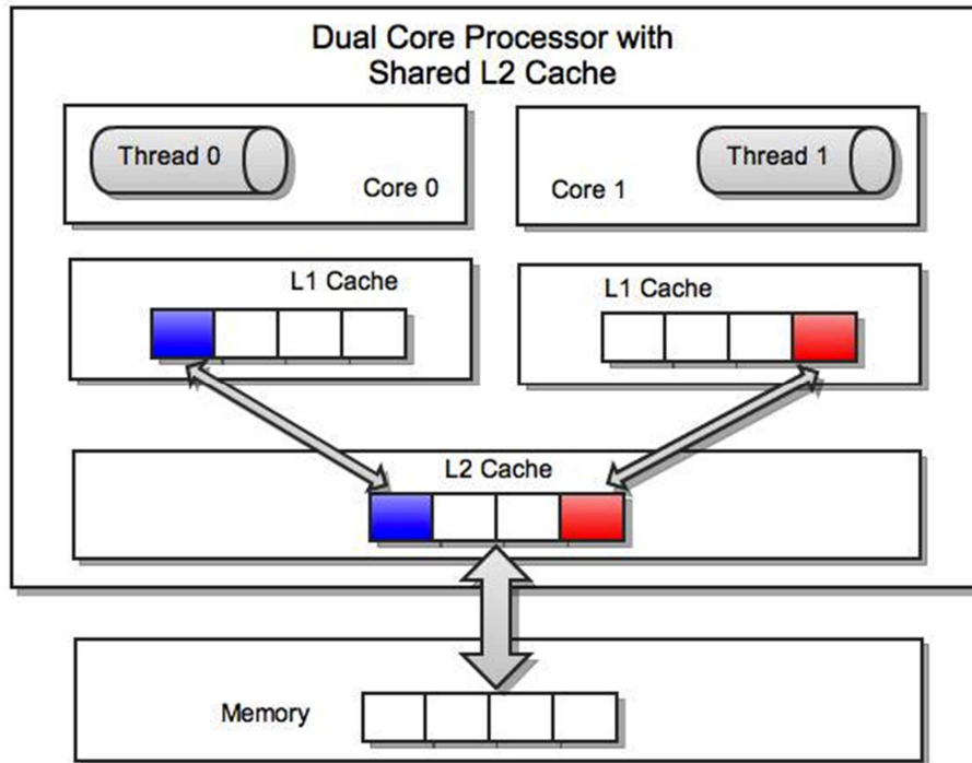
Figure 5. False cache line sharing on CMP [7]
