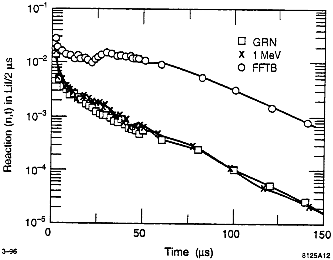
Fig. 4.3c. MCNP-calculated neutron arrival time distribution in the 2" Bonner Sphere detector for GRN and FFTB measured neutron spectrum compared with that for 1 MeV neutrons.
