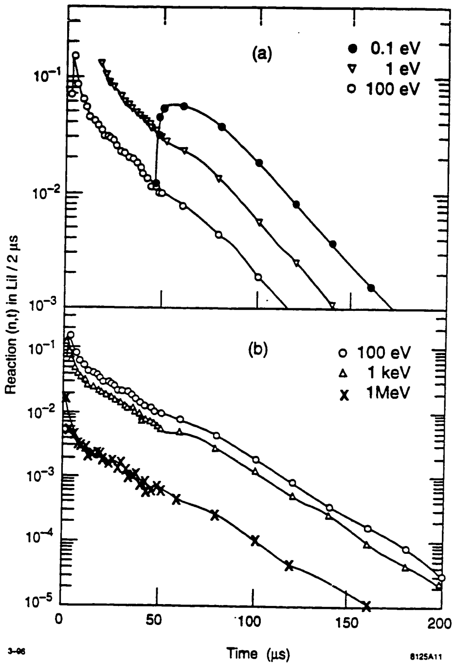
Figs. 4.3a and b. MCNP-calculated neutron arrival time distribution in the 2" Bonner Sphere detector for monoenergetic neutrons. (a) for 0.1 eV - 100 eV (b) for 100 eV - 1 MeV.
