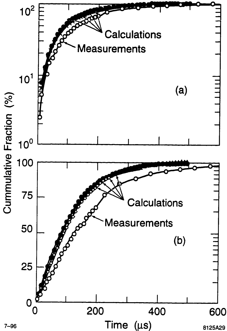
Figs. 4.9a and b A comparison between the MCNP-calculations and the measurement of fractional cumulative counts versus the neutron arrival time for the FFTB spectrum incident on the moderated BF 3 detector (a) a semilog plot (b) a linear plot. The calculations include the results for three GRN spectra (for a=1 MeV, a=1.2 MeV, and a=0.8 MeV) and the measured FFTB neutron spectrum.
