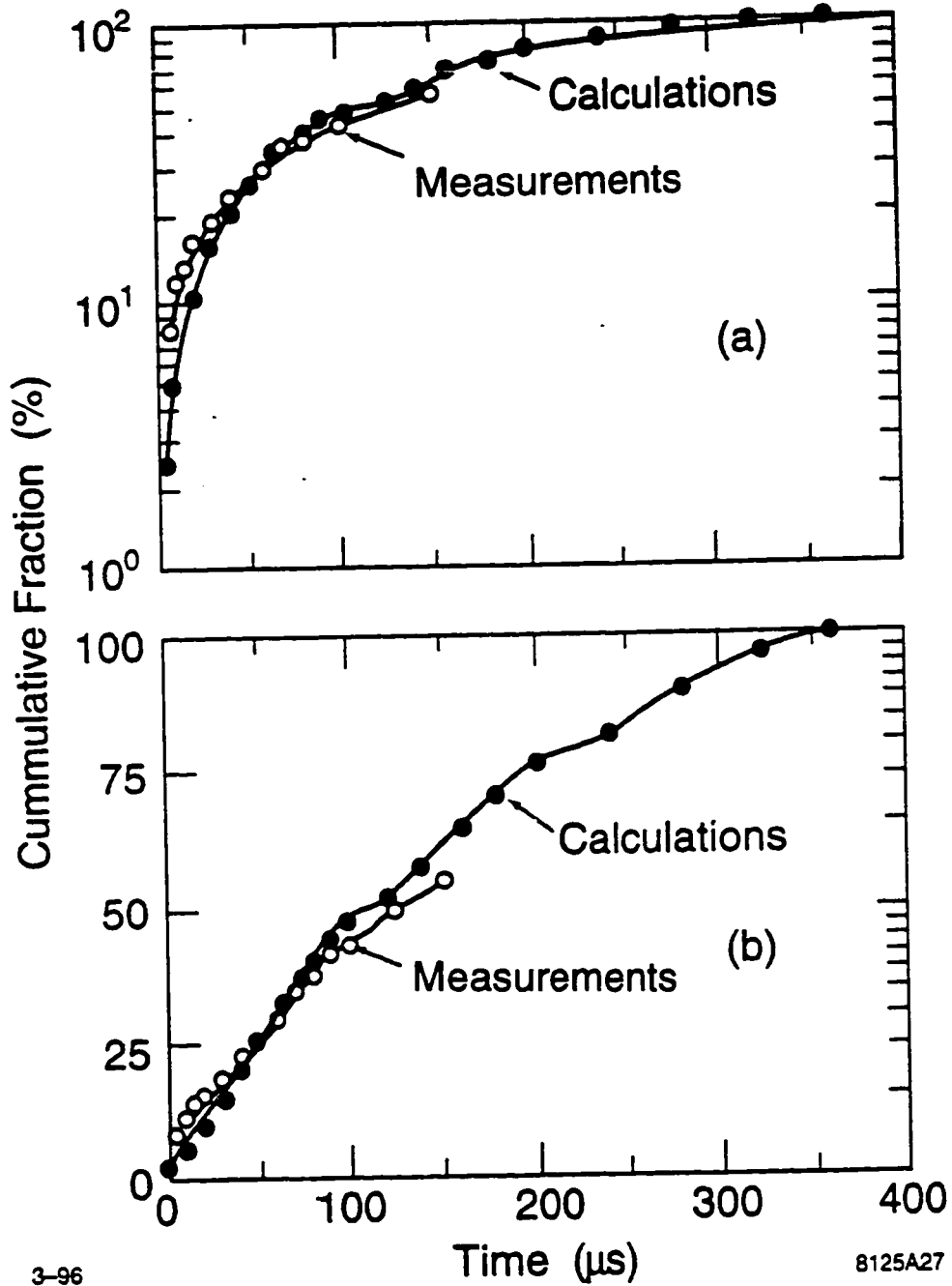
Figs. 4.12a and b A comparison between the MCNP-calculations and the measurement of fractional cumulative counts versus the neutron arrival time for the FFTB spectrum incident on the 10" Bonner Sphere detector (a) a semilog plot (b) a linear plot.
