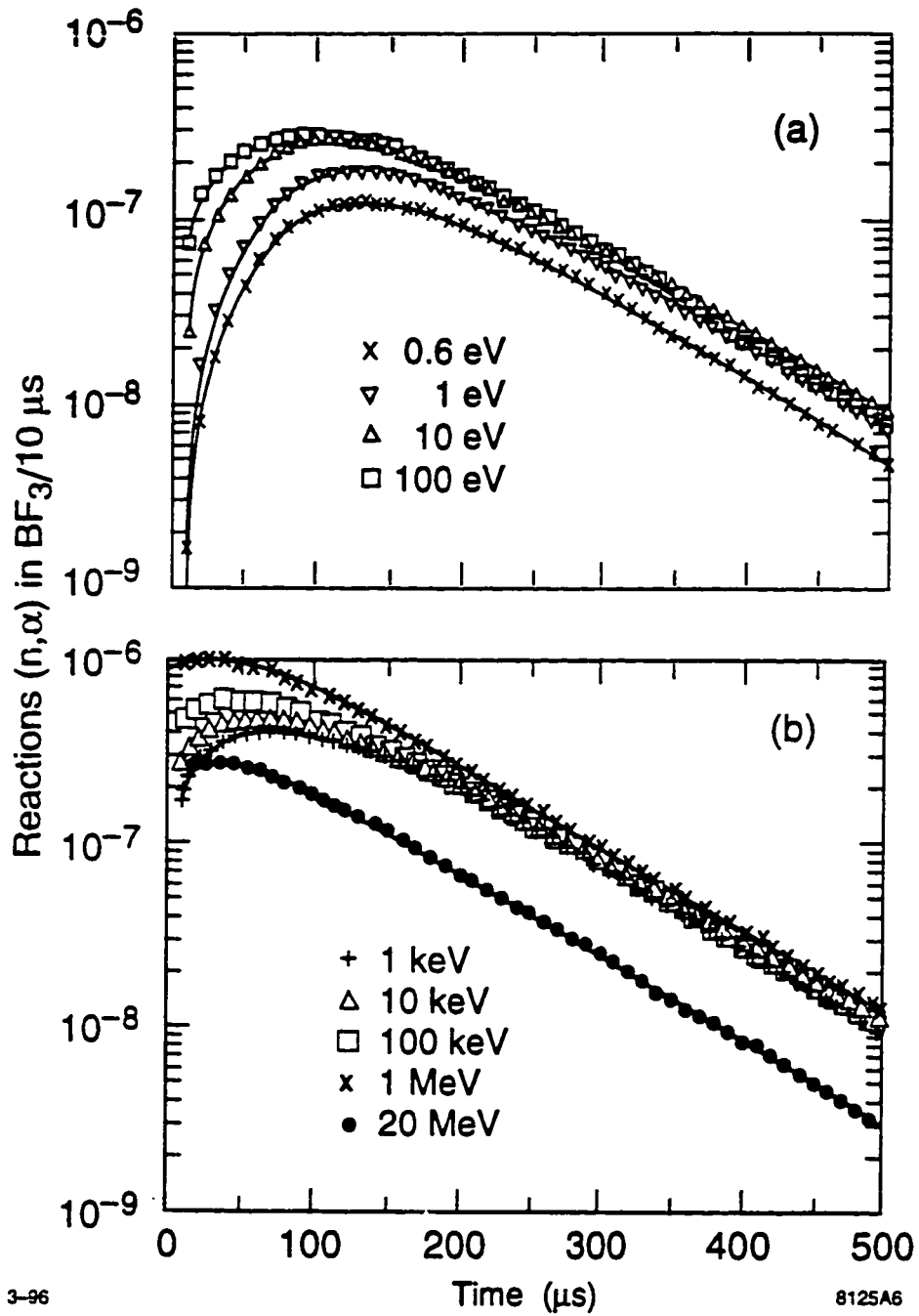
Figs. 4.1 a and b MCNP-calculated neutron arrival time distribution in the moderated \text{BF}_3 detector for monoenergetic neutrons. (a) for 0.6 eV - 100 eV (b) for 1 keV - 20 MeV.
