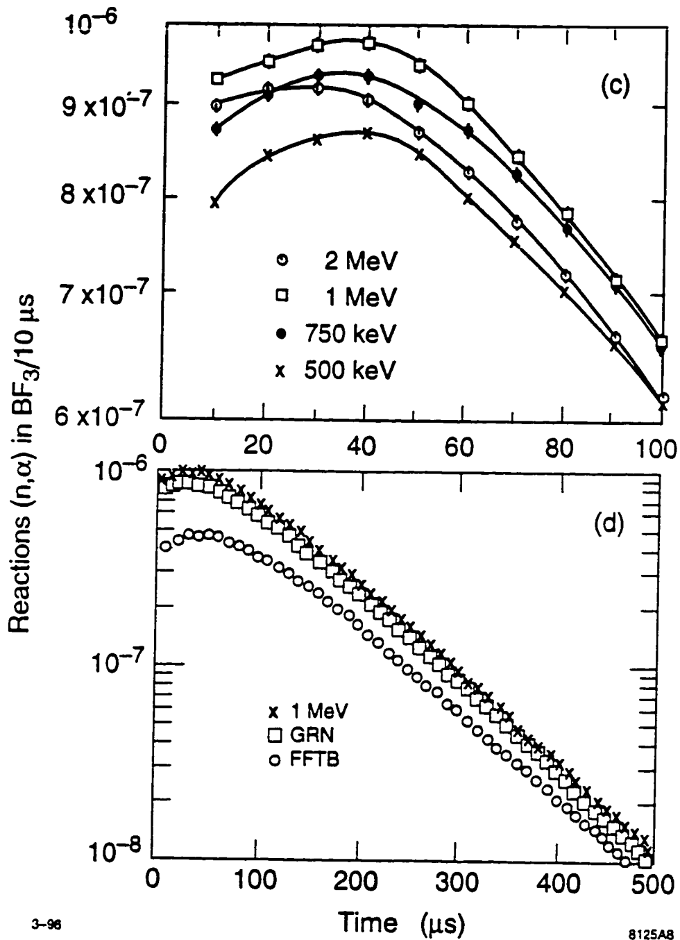
Figs. 4.1 c and d. MCNP-calculated neutron arrival time distribution in the moderated \text{BF}_3 detector (c) 500 keV - 2 MeV (d) for GRN and FFTB measured neutron spectrum.
