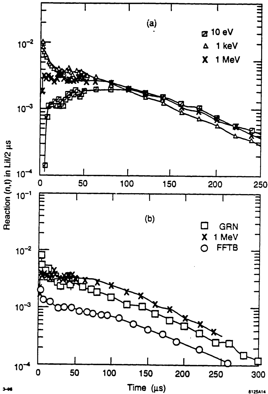
Figs. 4.5a and b MCNP-calculated neutron arrival time distribution in the 5" Bonner Sphere detector (a) for monoenergetic neutrons (b) for GRN and FFTB measured neutron spectrum compared with that for 1 MeV neutrons.
