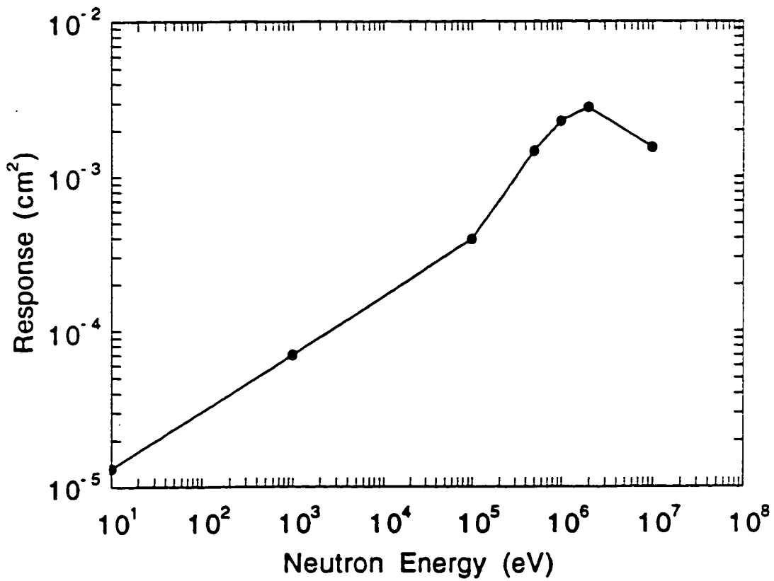
Fig. 4.2d. MCNP-calculated response of the Anderson-Braun remmeter . Note that the counts are per unit fluence.
