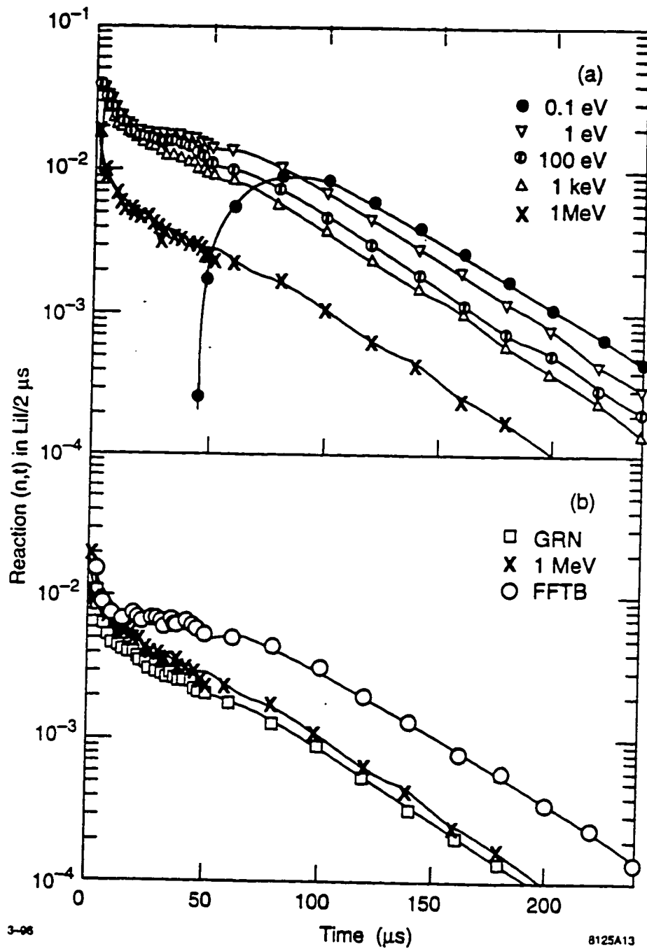
Figs. 4.4a and b. MCNP-calculated neutron arrival time distribution in the 3" Bonner Sphere detector (a) for monoenergetic neutrons (b) for GRN and FFTB measured neutron spectrum compared with that for 1 MeV neutrons.
