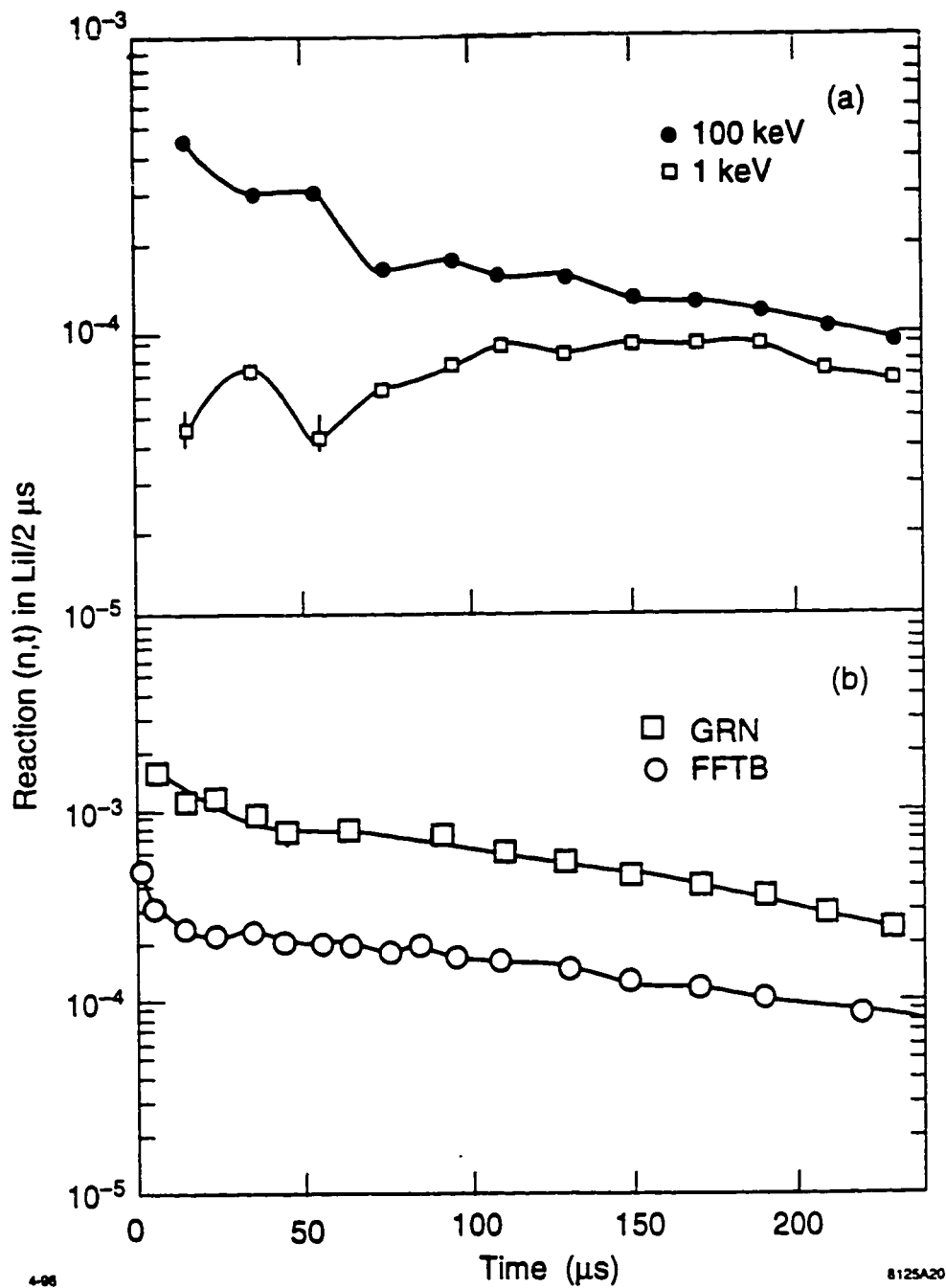
Figs. 4.6a and b MCNP-calculated neutron arrival time distribution in the 8" Bonner Sphere detector (a) for monoenergetic neutrons (b) for GRN and FFTB measured neutron spectrum.
