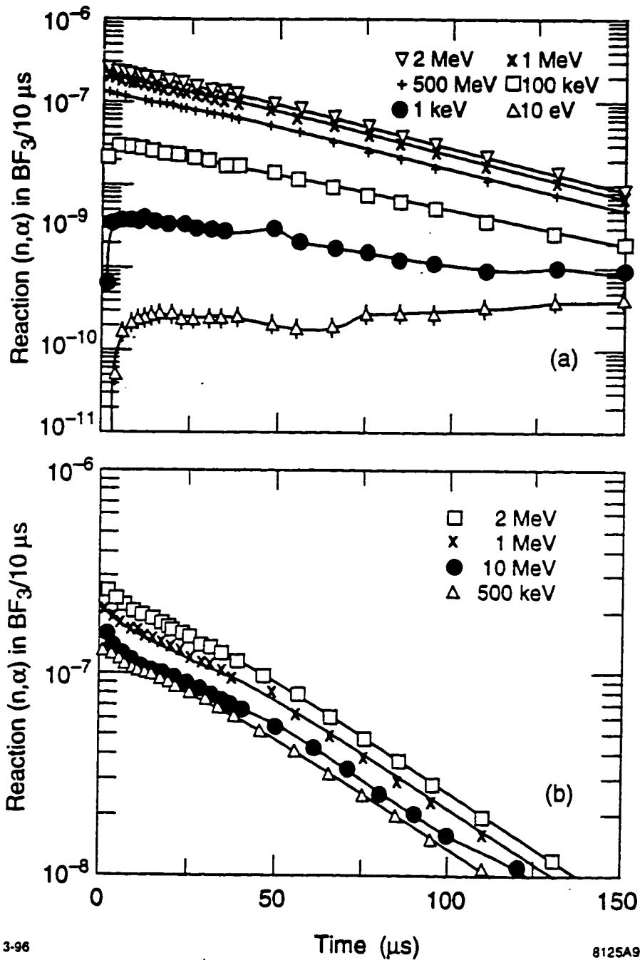
Figs. 4.2a and b. MCNP-calculated neutron arrival time distribution in the Anderson-Braun remmeter for monoenergetic neutrons.(a) for 10 eV - 2 MeV (b) for 500 keV - 10 MeV.
