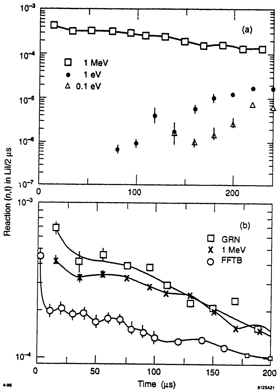
Figs. 4.7a and b MCNP-calculated neutron arrival time distribution in the 10" Bonner Sphere detector (a) for monoenergetic neutrons.(b) for GRN and FFTB measured neutron spectrum compared with that for 1 MeV neutrons.
