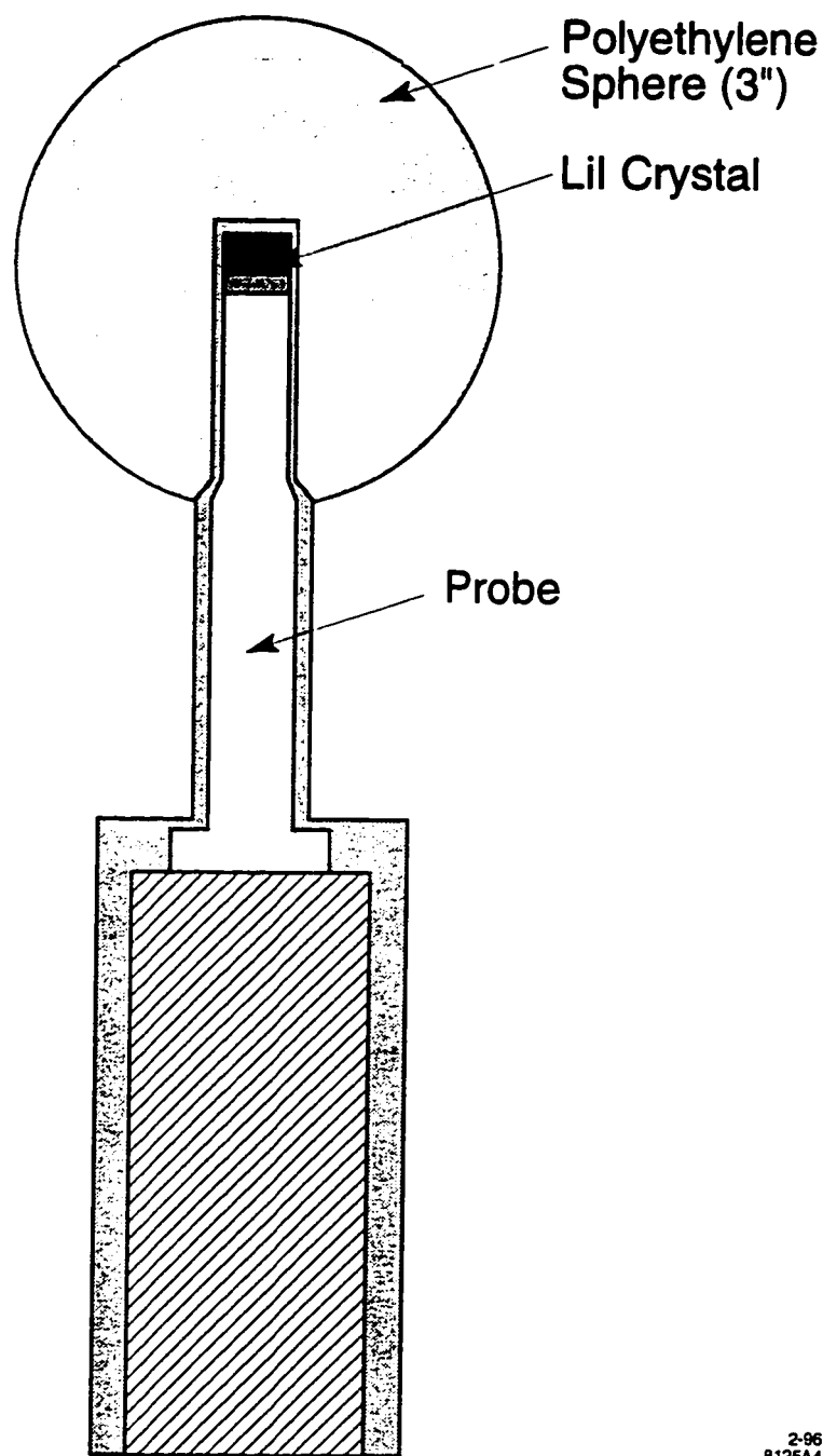
Fig. 2.3b Schematic representation of cross-section of the Bonner Sphere detector assembly.
