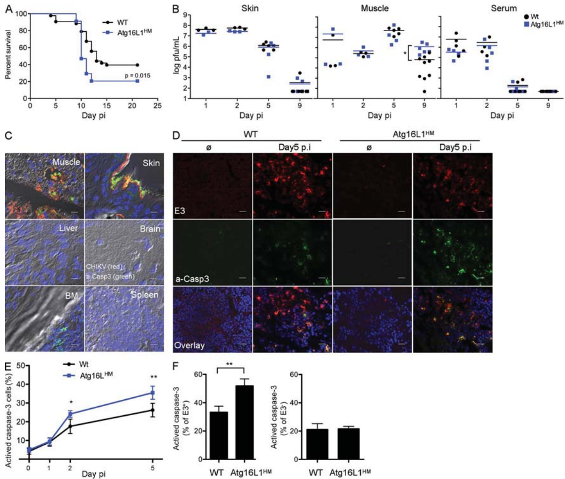
Figure 8. Autophagy limits apoptotic induction in CHIKV infected tissues and delays lethality of mice. (A–F) WT ( n = 43 ) and Atg16L1 HM mice ( n = 34 ) were infected at 9 d of age with 4 \times 10^5 PFU CHIKV subcutaneously. (A) Mice were monitored for lethality for 21 d with data displayed as Kaplan–Meier curves. (B) Skin, muscle, and serum were collected after days 1 ( n = 3 ), 2 ( n = 3 ), 5 ( n = 4 ), and 9 ( n = 5 ) of infection, homogenized, and viral titers were determined by standard plaque assay. Median values for WT (black bars) or Atg16L1 HM (blue bars) mice are depicted. (C) Muscle, skin, liver, brain, BM, and spleen were collected from WT infected mice at day 5. Tissues were fixed in PFA, frozen in OCT blocks, and stained for cleaved caspase-3 (green) and E3 (red). Similar results were observed in two independent experiments. Bars: (muscle) 50 \mu m; (other tissues) 20 \mu m. (D–F) Muscle from infected WT or Atg16L1 HM mice was collected at days 1, 2, and 5 after infection and stained for cleaved caspase-3, E3, or DAPI for nucleus staining (D). The percentage of cleaved caspase-3–positive cells was numerated in all population (E) or in E3 + and E3 – cells (F). Error bars mean \pm SD of three independent experiments. Bars, 60 \mu m. Student's test: **, P < 0.05 .
