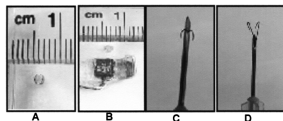
FIG. 1. Experimental equipment. (A) Neodymium magnetic disk and (B) GMR sensor. (C) and (D) Bipolar EMG wire electrodes mounted on hyperdermic needle.
