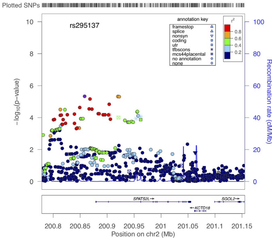
Figure 2. Region of association near SPATS2L SNPs to BDR. The x-axis denotes position along Chromosome 2. The y-axis denotes -\log_{10}(P) corresponding to 1000GP imputed data P-values. LD between the SNP with the lowest P-value (rs295137) to each SNP in the plot is denoted in colors and was computed according to 1000GP June 2010 CEU data. Plot was created using LocusZoom [44]. doi:10.1371/journal.pgen.1002824.g002
