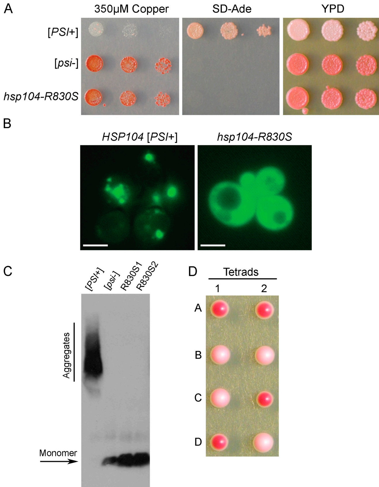
Figure 1. hsp104-R830S propagates cryptic [PSI+]. (A) [PSI+], [psi-], and hsp104-R830S cells were spotted on media containing \text{CuSO}_4 to induce toxic overexpression of Sup35, media lacking adenine (SD-Ade) to assess nonsense suppression of the premature stop codon in ade1-14 , and rich media (YPD). (B) HSP104 [PSI+] and hsp104-R830S cells containing pSup35NM-GFP were imaged by fluorescence microscopy. Bar, 10 \mu\text{m} . (C) Western blot of an SDS-containing agarose gel (SDD-AGE) shows Sup35 aggregate status in lysates of indicated strains. This blot is one representative of three individual experiments. (D) An example of two tetrads where mating hsp104-R830S to [psi-] cells, both containing the ade1-14 mutation, resulted in tetrads with two red (efficient translation termination, hsp104-R830S ) and two light pink (increased nonsense suppression, [PSI+] HSP104 ) haploids.
