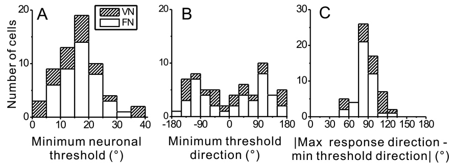
Figure 5. Summary of neuronal thresholds. A , Distribution of minimum neuronal thresholds for 41 FN and 20 VN cells. B , Distribution of reference heading directions for which minimum neuronal thresholds were obtained. C , Distribution of the difference between minimum threshold direction and the maximum response direction. Open bars, FN cells; striped bars, VN cells.
