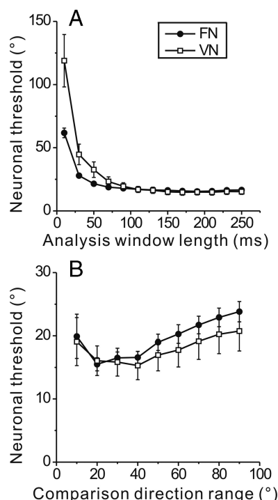
Figure 8. A , Dependence of neuronal thresholds on the length of the time window (centered on the middle of each response half-cycle) in which firing rates were computed. B , Dependence of thresholds on the range of comparison headings used to construct the neurometric function using ROC analysis. This dependence is illustrated for the reference heading that produced the minimum threshold for each neuron using a time interval of 250 ms and a 40 ^{\circ} heading range. Filled symbols, FN cells ( n = 41 ); open symbols, VN cells ( n = 20 ). Data illustrate mean \pm SE.
