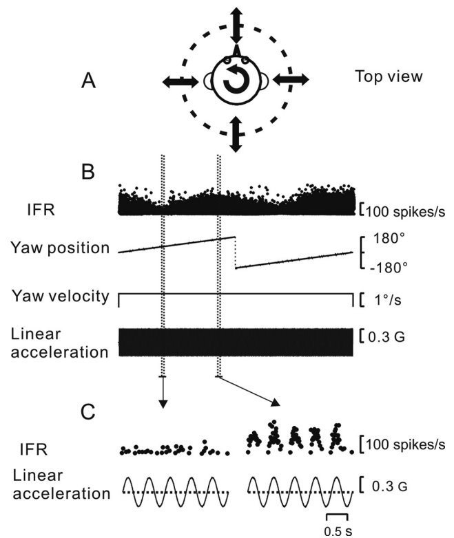
Figure 1. Experimental protocol and neuronal responses. A , Schematic of the continuous linear acceleration stimulus around the head horizontal plane. B , IFR of a FN cell during combined sinusoidal translation (2 Hz; \pm 0.3 G) and constant velocity rotation (1°/s). C , Enlarged time scale near the minimum and maximum response modulation, respectively.
