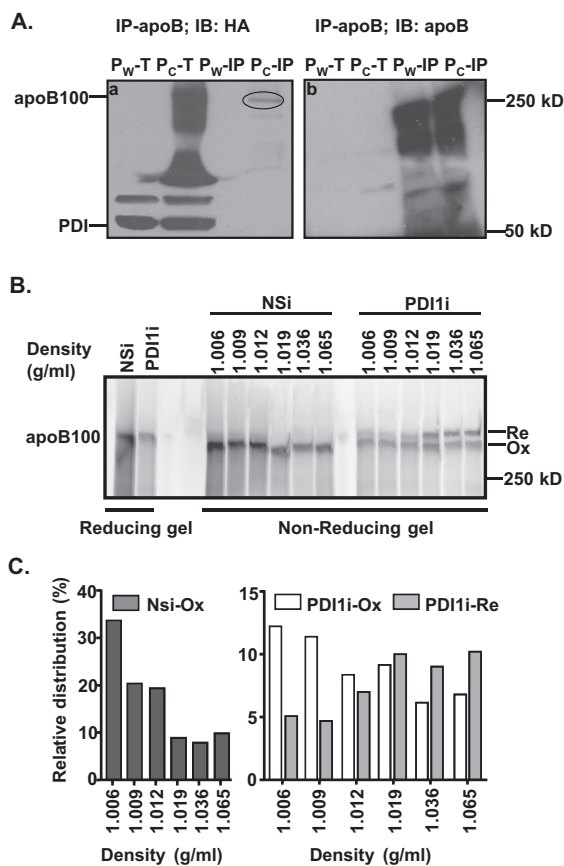
FIGURE 5: Reduced apoB100 oxidative folding decreases apoB lipidation. (A) PDI1 forms intermolecular disulfide bond(s) with apoB100. Lysates from cells that stably express HA-tagged wild-type (Pw: HA-PDI1) or substrate-trap mutant (Pc: HA-PDI1 CXXA ) of human PDI1 were immunoprecipitated with apoB100 antibody and analyzed by nonreducing SDS-PAGE and immunoblotting against HA antibody. The circle indicates PDI1 complexed with apoB100. IP, immunoprecipitated protein complex; T, total cell lysates. (B) Impaired apoB100 oxidative folding decreases apoB100 lipidation. Secreted apoB100-containing lipoproteins from McA cells were separated by DGUC as described in Figure 3 and analyzed by nonreducing gel electrophoresis. (C) The amount of apoB100 in each fraction was quantified by ImageJ. Relative distributions were calculated according to the percentage of apoB100 in each fraction relative to its total intensity across the gel.
