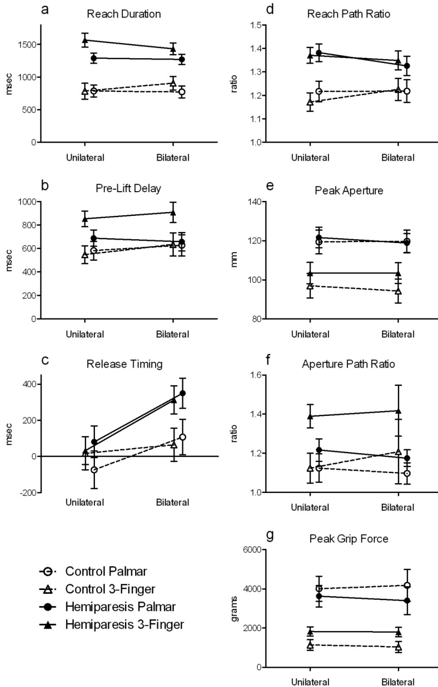
Fig. 2 Comparisons of reach-grasp-lift-release task performance when moving unilaterally versus bilaterally. Values are means \pm 1 standard error. The only variable that differed across the unilateral versus bilateral conditions was release timing (panel c). Participants in both groups released the object later when moving bilaterally instead of unilaterally. Refer to results section for effects of group and grip type.
