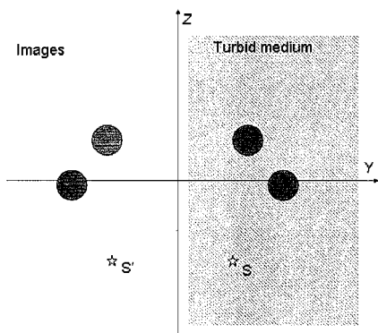
Fig. 10. Illustration of the method of images for the case of a single planar interface. The turbid medium, source, and spherical inhomogeneities are located in the right half-space. The mirror images of the inhomogeneities and source are in the left half-space.
