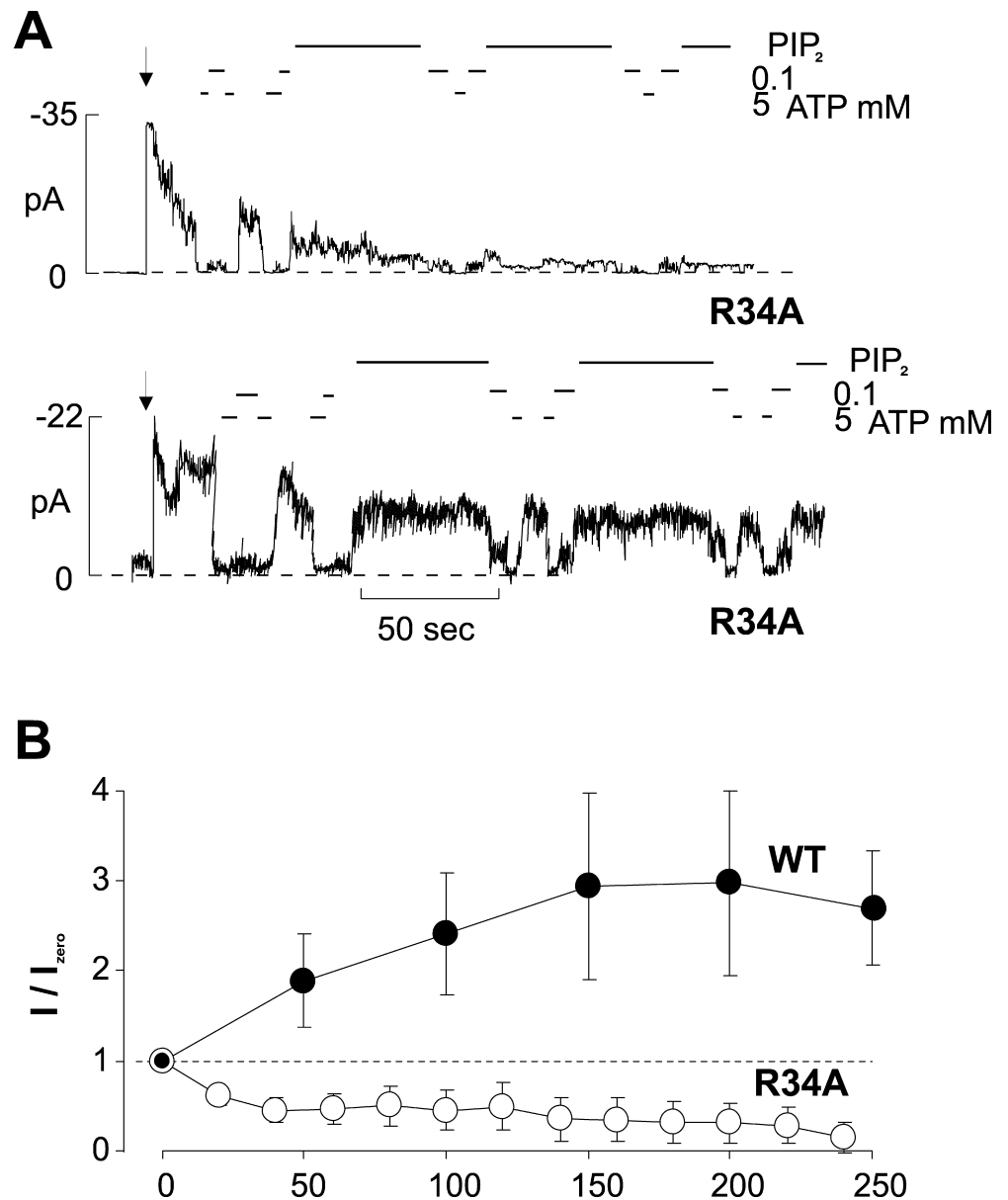
FIGURE 5. (A) Representative currents recorded from inside-out membrane patches containing Kir6.2[R34A] co-expressed with SUR1. The dashed line indicates zero current. (B) Mean current (in zero ATP) versus time after application of PIP 2 for Kir6.2 WT coexpressed with SUR1 and for Kir6.2[R34A] coexpressed with SUR1.
