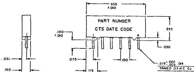
.100" centers (low profile)
