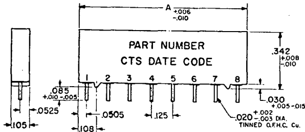
.125" centers
