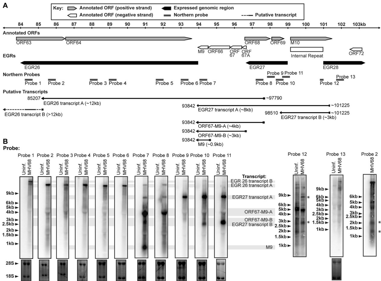
FIG 3 EGR 26 and 27 transcriptional architecture. (A) Schematic representation of EGR 26-27/M9 region transcripts. Approximate size and transcript name are listed below the relevant transcript. (B) Northern blot detection of EGR 26-27/M9 region transcripts. RNA harvested at 18 hpi (MOI = 10) was analyzed by Northern blot analysis using the indicated probes. 28S and 18S rRNA bands visualized by ethidium bromide staining to demonstrate equal loading are shown below the corresponding Northern blots. Northern blots analyzed with probe 12 and probe 2 (far right) had 500 ng of poly(A)-selected RNA per lane. *, virus-specific bands that are of comparable size to EGR 27 transcripts A and B. **, smaller EGR 26 transcripts referenced in text.
