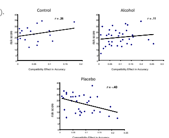
Figure 6. Correlations between Risk Score and CE_acc.
