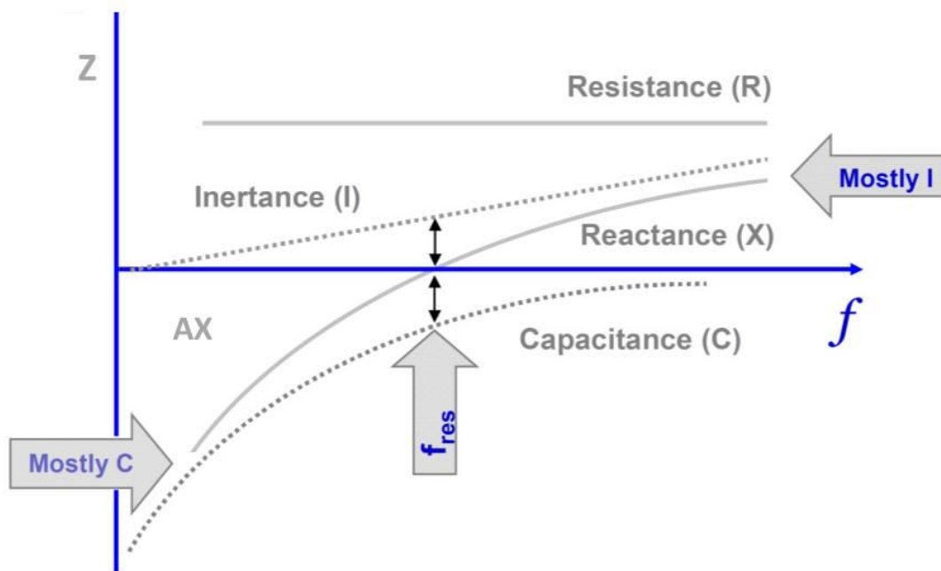
Figure 4. Schematic illustration of components of impedance ( Z ) in a healthy subject with absent frequency dependence of resistance ( by courtesy of Per Gustafsson)
