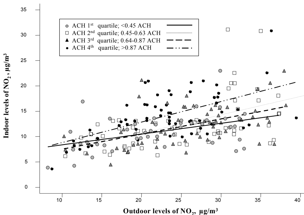
Figure 4. Correlation between outdoor and indoor \text{NO}_2 levels in homes, without internal sources of \text{NO}_2 , with the regression lines for different quartiles of measured air change rate
