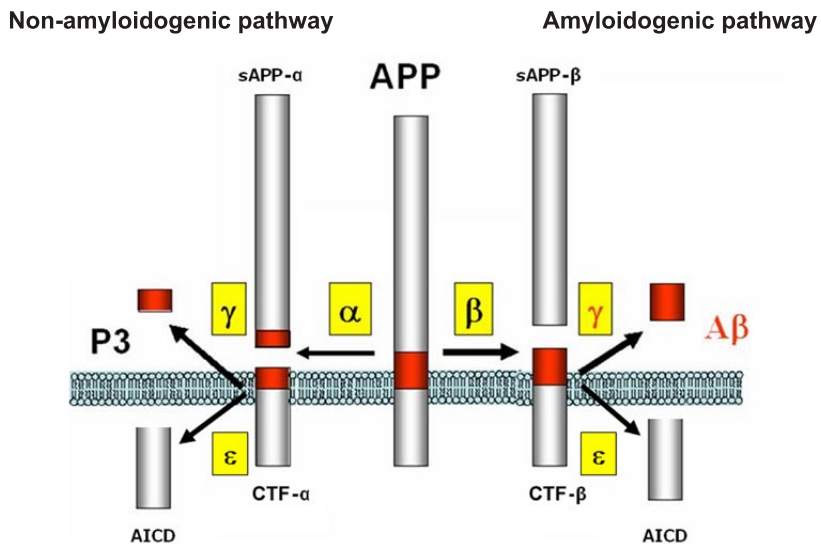
Figure 2. Schematic overview of the general processing of the amyloid precursor protein; the non-amyloidogenic pathway constitutes a ‘non-A \beta ’ pathway, with a cleavage within the A \beta region, whereas the amyloidogenic pathway generates A \beta peptide of lengths between 39–42 amino acids.
