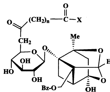
PF hemiglutarate-BSA conjugate: X = \text{BSA} \dots \text{NH} , n = 3 PF hemisuccinate- \beta -Gal conjugate: X = \beta\text{-Gal} \dots \text{NH} , n = 2
