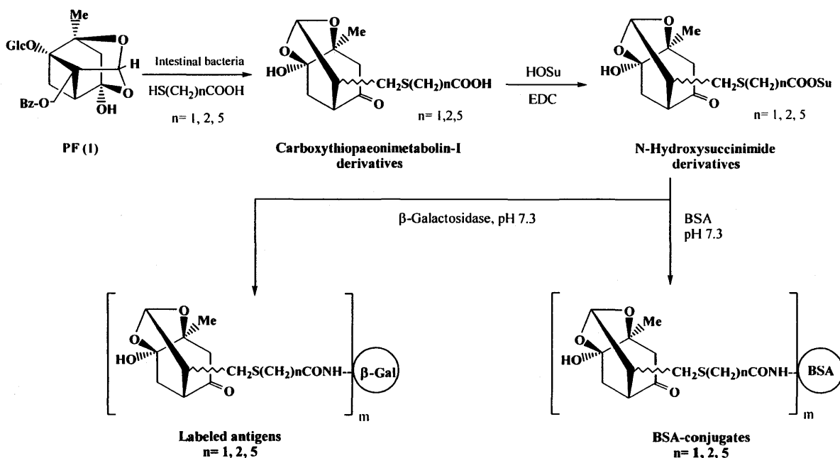
Chart 6. BSA- and \beta -Gal-conjugates of paeonimetalolin-I
