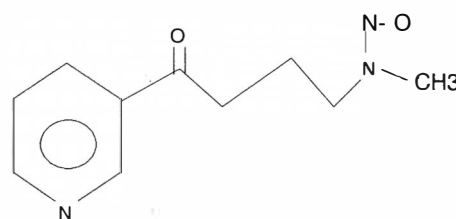
4-(Methylnitrosamino)-1-(3-pyridyl)-1-butanone (NNK)
