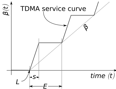
Figure 2: TDMA service curve
