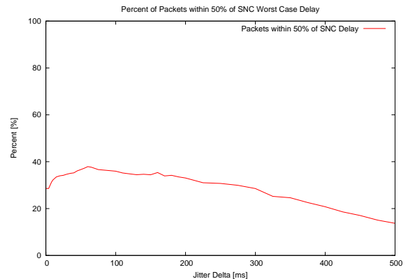
Figure 8: Percentage of messages with 455ms < d_i < 890ms .
