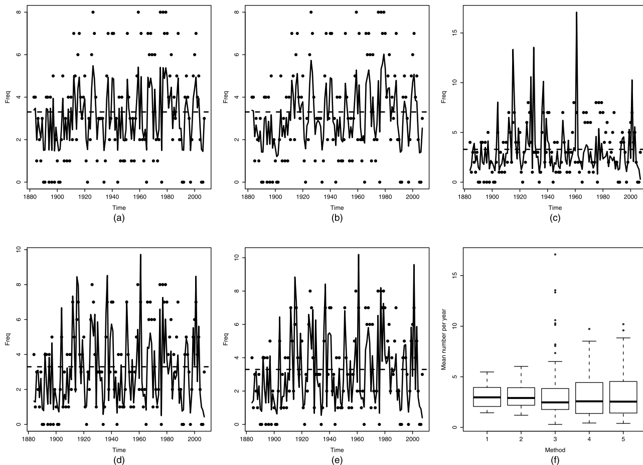
Figure 3. (a–e) Estimated expected annual counts (lines) for all five fitted models. Observed numbers of events are shown by dots, and the overall sample mean is shown by a horizontal dashed line. (f) Box plots of these estimated expected annual counts.
