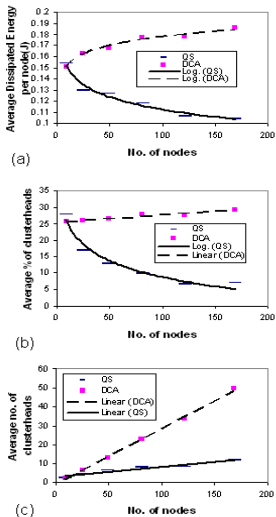
Figure 9(a): The average energy dissipated by a node in the network of increasing size, (b) the average percentage of cluster-heads per minute and (c) the average number of cluster-heads when running the QS and DCA algorithm
