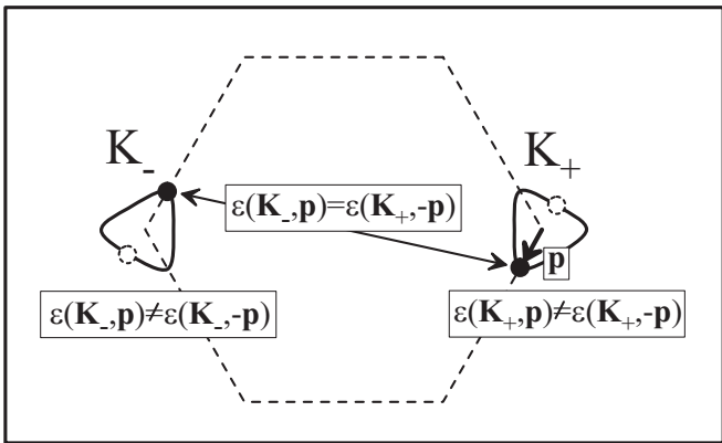
FIG. 1: Fermi lines (solid lines) in the vicinity of two inequivalent valleys \mathbf{K}_+ and \mathbf{K}_- of the hexagonal Brillouin zone (dashed line). Trigonal warping produces asymmetry of the dispersion at each valley \epsilon(\mathbf{K}_\pm, \mathbf{p}) \neq \epsilon(\mathbf{K}_\pm, -\mathbf{p}) , where momentum \mathbf{p} is determined with respect to the center of the valley, but the effects of warping in the valleys have opposite signs, \epsilon(\mathbf{K}_\pm, \mathbf{p}) = \epsilon(\mathbf{K}_\mp, -\mathbf{p}) . The bilayer lattice configuration is described in detail in [12].
