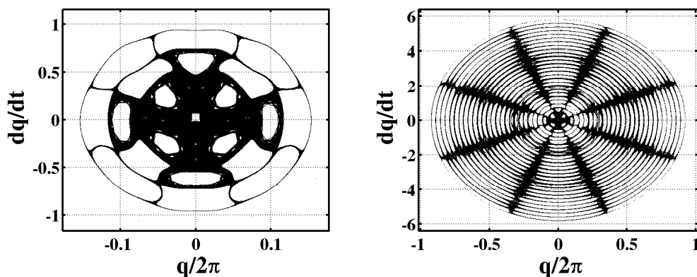
FIGURE 1. The Poincaré section for a trajectory of the system (1) with initial state q = 0.1 , \dot{q} = 0 (at instants t_n = nT where T \equiv 2\pi/0.02 is the period of the modulation and n = 1, 2, 3, \dots, 600000 ) for h = 0 (left panel) and h = 0.1 (right panel). A symplectic integration scheme of the fourth order is used, with an integration step t_{int} = \frac{2\pi}{40000} \approx 1.57 \times 10^{-4} , so that the inaccuracy at each step is of the order of t_{int}^5 \approx \times 10^{-19} . The left panel corresponds to the conventional case considered in [1, 4, 6]. The right panel demonstrates that the modulation, although weak, greatly enlarges the web sizes (note the different axes scales), thereby greatly enhancing the chaotic transport.
