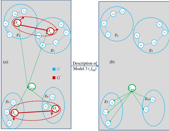
Fig. 5. Model 3: (a) use graph structure \mathbf{G}' by calculating the distance from the new node v_{new} to the centres of all groups. Once one group g_i satisfies the distance threshold, (b) calculate the distances between v_{new} and any node in g_i in addition to the distance between v_{new} and any node in a group connected to g_i through \mathbf{G}' .
