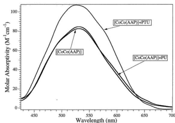
Figure 3 Electronic absorption spectra of 1 mM [CoCo(AAP)] in 50 mM HEPES buffer at pH 7.5 recorded in the presence and absence of PTU and PU. The electronic absorption spectrum of apo-enzyme was subtracted in each case.
