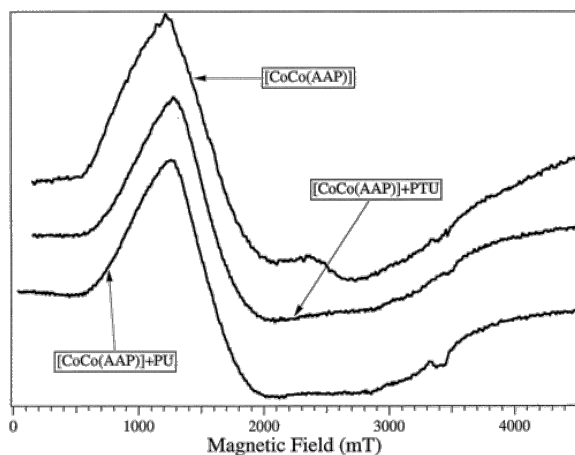
Figure 5 EPR spectra of 1 mM [CoCo(AAP)] in 50 mM HEPES buffer at pH 7.5 recorded in the presence and absence of PTU and PU. All spectra were recorded using 100 kHz modulation frequency, 1.26 mT modulation amplitude, 3.12 \text{ mT s}^{-1} field sweep rate, and 164 ms time constant.
