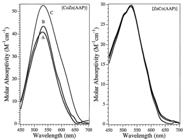
Figure 4 Electronic absorption spectra of 1 mM [CoZn(AAP)] (left panel) and [ZnCo(AAP)] (right panel) in 50 mM HEPES buffer at pH 7.5 recorded in absence (A) and presence of PU (B) and PTU (C). The electronic absorption spectrum of apo enzyme was subtracted in each case.
