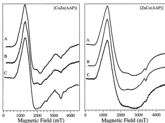
Figure 6 EPR spectra of [CoZn(AAP)] (left panel) and [ZnCo(AAP)] (right panel) in 50 mM HEPES buffer at pH 7.5 recorded in the absence (A) and presence of PU (B) and PTU (C). All spectra were recorded using 100 kHz modulation frequency, 1.26 mT modulation amplitude, 3.12 mT s -1 field sweep rate, and 164 ms time constant.
