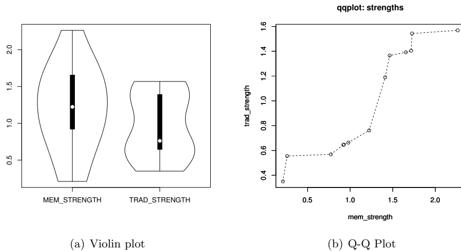
Figure 5-16: Password strengths
