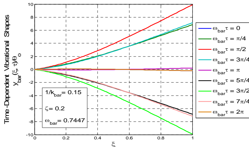
Figure 6-15: Time-dependent vibrational shapes due to relative harmonic rotation near support for 1/\bar{k} = 0.15 , \zeta = 0.2 , and \bar{\omega} = 0.7447 .
