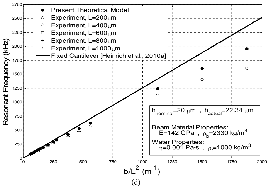
Figure 6-16: Fundamental lateral resonant frequency comparisons: current model, fixed cantilever model [Heinrich et al., 2010a], and experimental data for the following nominal Si thicknesses: (a) 5\mu\text{m} ; (b) 8\mu\text{m} ; (c) 12\mu\text{m} ; (d) 20\mu\text{m} .
