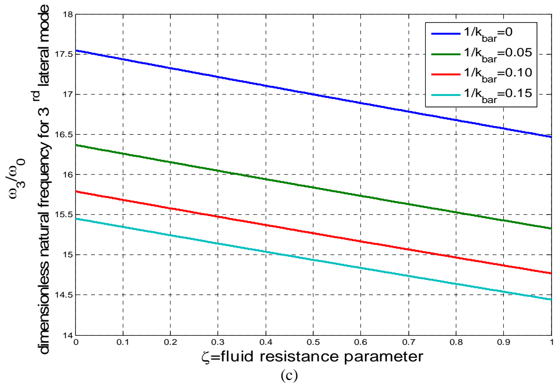
Figure 6-1: Dimensionless natural frequency for the first three modes of lateral vibration of a microcantilever beam in a viscous fluid [Eq. (4-18)]: (a) first mode, (b) second mode, (c) third mode.
