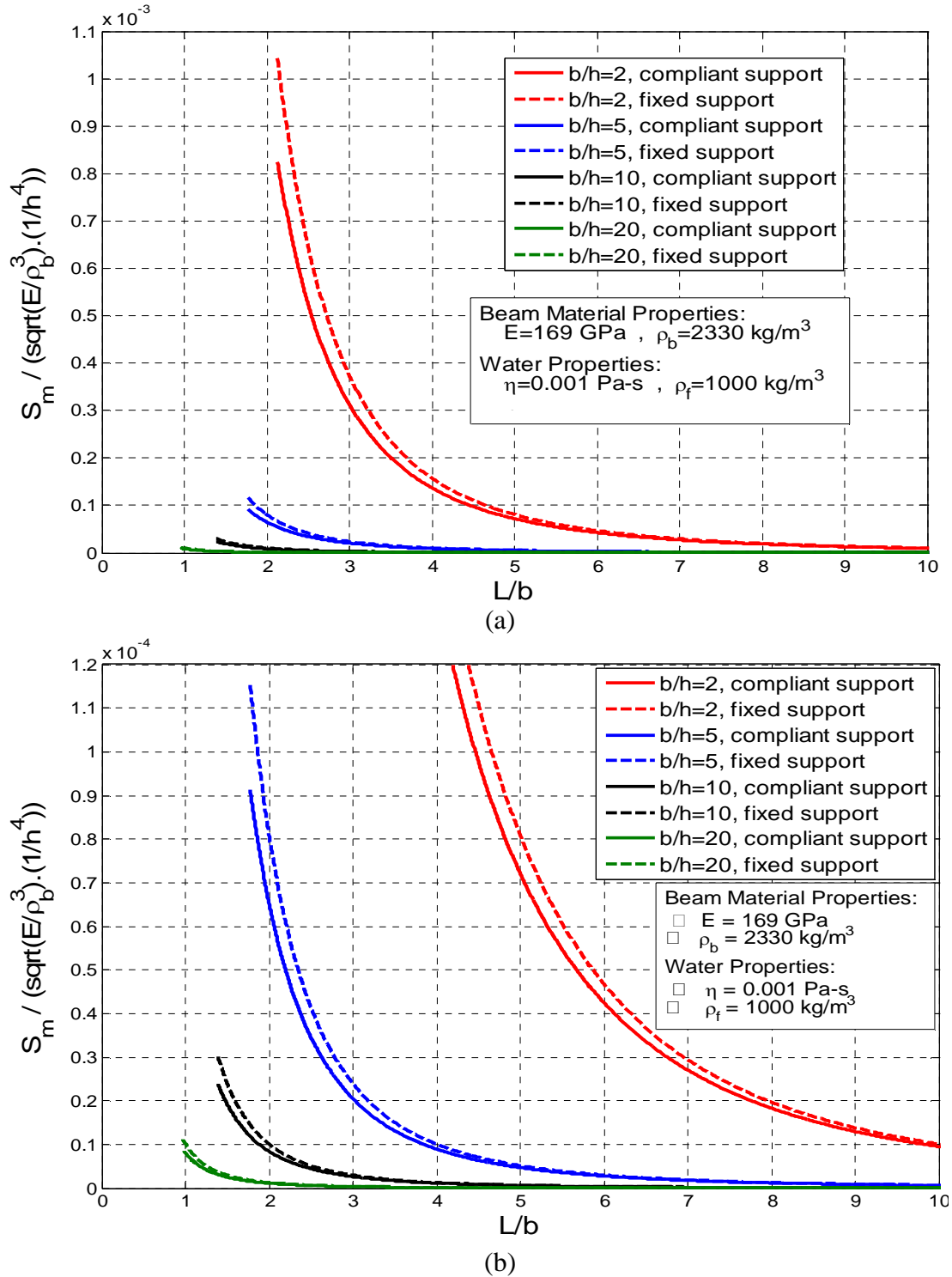
Figure 7-1: Normalized mass sensitivity of laterally vibrating silicon microcantilevers with h > 5 \mu\text{m} in water: (a) S_m / \sqrt{\frac{E}{\rho_b^3}} \frac{1}{h^4} \in [0, 0.0011] ; (b) S_m / \sqrt{\frac{E}{\rho_b^3}} \frac{1}{h^4} \in [0, 0.00012] (zoomed view). These figures should NOT be applied for L/b ratios in excess of the upper bound listed in Eq. (6-2).
