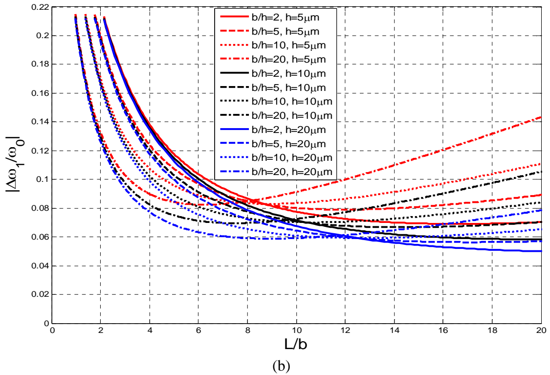
Figure 6-3: Relative difference between fundamental lateral natural frequency and perfectly clamped in-vacuum value for a silicon microcantilever beam in water with h = [5, 10, 20] \mu\text{m} and b/h = [2, 5, 10, 20] : (a) L/b \in [0, 160] , (b) L/b \in [0, 20] (zoomed view).
