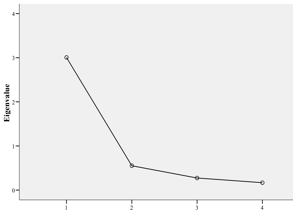
Figure 3. Scree plot, ECLS-K mathematics self-concept items
