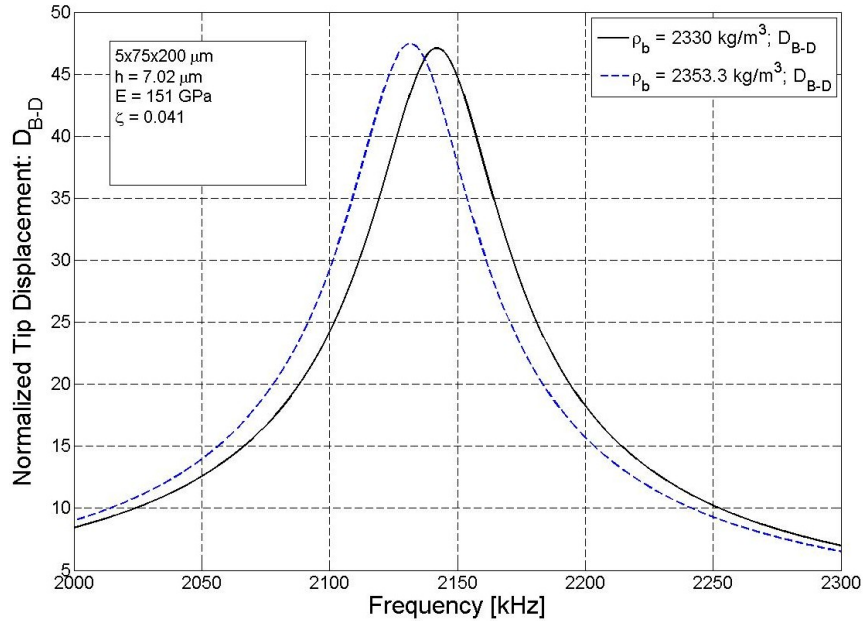
Figure 5-1: Shift in Frequency Response Curve Due to 1% Increase in Beam Density to Mirror the Effect of Analyte Sorption by a 5 x 75 x 200 \mu\text{m} Microcantilever-Based Sensor in Water: \rho_f = 1000 \text{ kg/m}^3 and \eta = 0.001 \text{ Pa}\cdot\text{s} . Measured by the Bending-Deformation Displacement of the Response Due to a Harmonic Support Rotation
