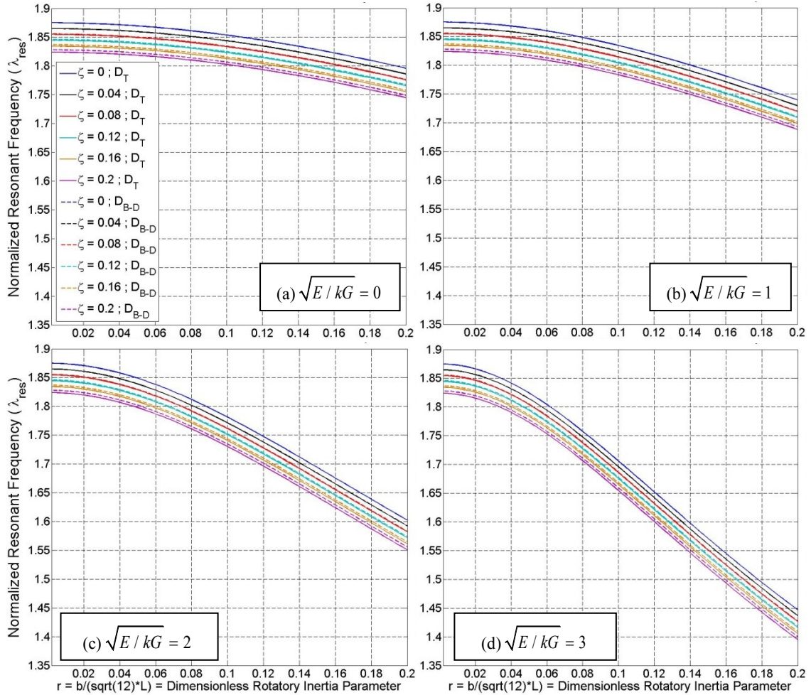
Figure 4-16: Resonant Frequency at Tip ( \xi=1 ) for Various Fluid Resistance parameters ( \zeta ), for r = b / (L\sqrt{12}) \in [0, 0.2] Measured by D_T and D_{B-D} : (a) \sqrt{E/kG} = 0 , (b) \sqrt{E/kG} = 1 , (c) \sqrt{E/kG} = 2 , (d) \sqrt{E/kG} = 3
