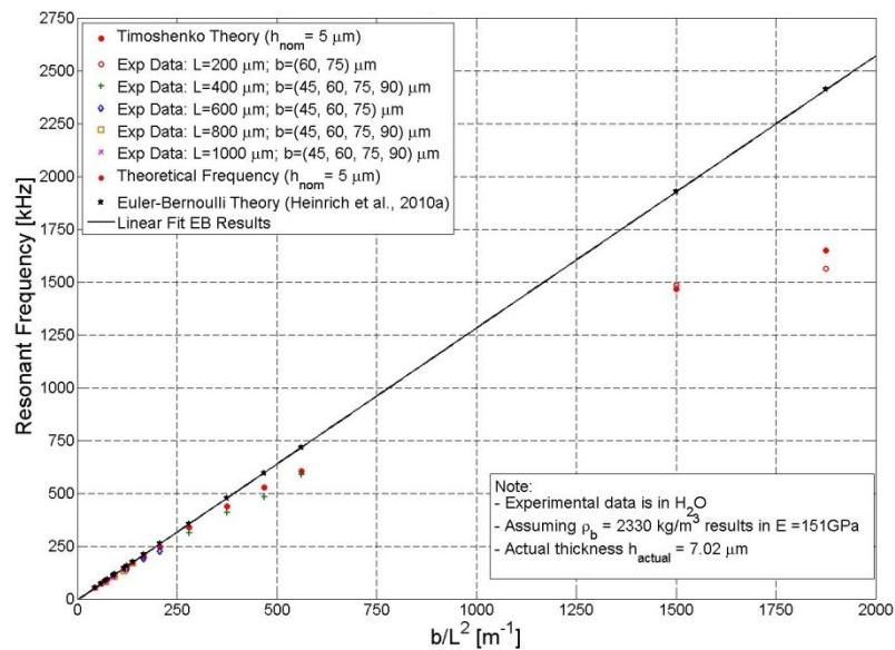
Figure 4-30: Comparison of Current In-Fluid, Timoshenko Model to Experimental [Beardslee et al., 2010d] In-Fluid Resonant Frequencies For First Lateral Flexural Mode Due to Harmonic Support Rotation; Nominal Thickness of 5 \mu\text{m} , \sqrt{E / 12\rho_b} = 2.3240 \text{ km/sec} , \sqrt{E / kG} = 4.4231 and E = 151 \text{ GPa}
