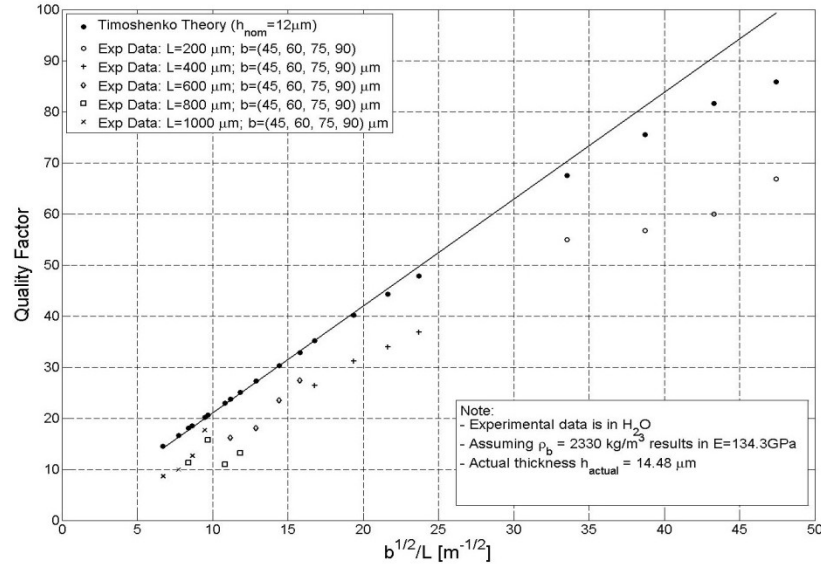
Figure 4-40: Comparison of Current In-Fluid, Timoshenko Model to Experimental [Beardslee et al., 2012] Quality Factor for First Lateral Flexural Mode, Nominal Thickness 12 \mu\text{m} Using \sqrt{E / 12\rho_b} = 2.1920 \text{ km/sec} and \sqrt{E / kG} = 3.1288
