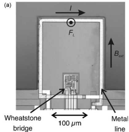
Figure 1-1: Image of Conventional Microcantilever-based Chemical Sensor with Wheatstone Bridge and Metal Loop for Transverse Actuation [Vancura et al., 2008]
