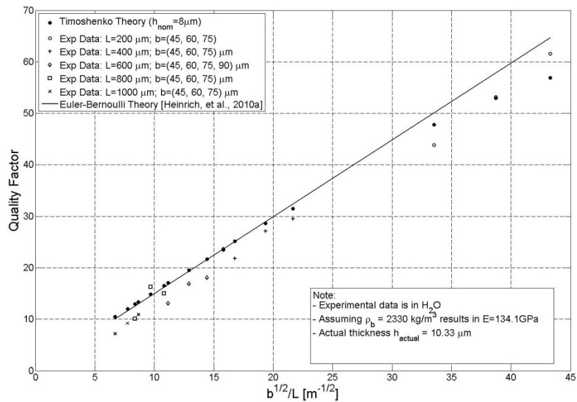
Figure 4-39: Comparison of Current In-Fluid, Timoshenko Model to Experimental [Beardslee et al., 2012] Quality Factor for First Lateral Flexural Mode, Nominal Thickness 8 \mu m Using \sqrt{E / 12\rho_b} = 2.1903 \text{ km/sec} and \sqrt{E / kG} = 3.511667
