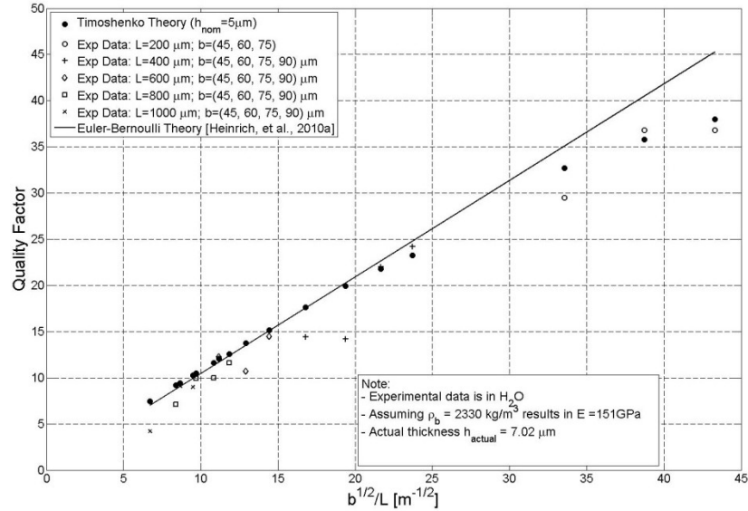
Figure 4-38: Comparison of Current In-Fluid, Timoshenko Model to Experimental [Beardslee et al., 2012] Quality Factor for First Lateral Flexural Mode, Nominal Thickness 5 \mu m Using \sqrt{E / 12\rho_b} = 2.3240 \text{ km/sec} and \sqrt{E / kG} = 4.4231
