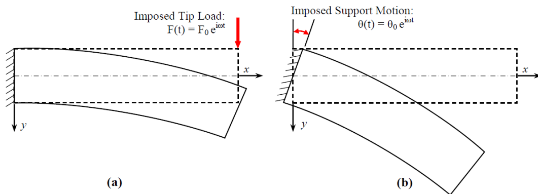
Figure 1-5: (a) Load Case 1 – Imposed Harmonic Tip Load (b) Load Case 2 – Imposed Harmonic Support Rotation
