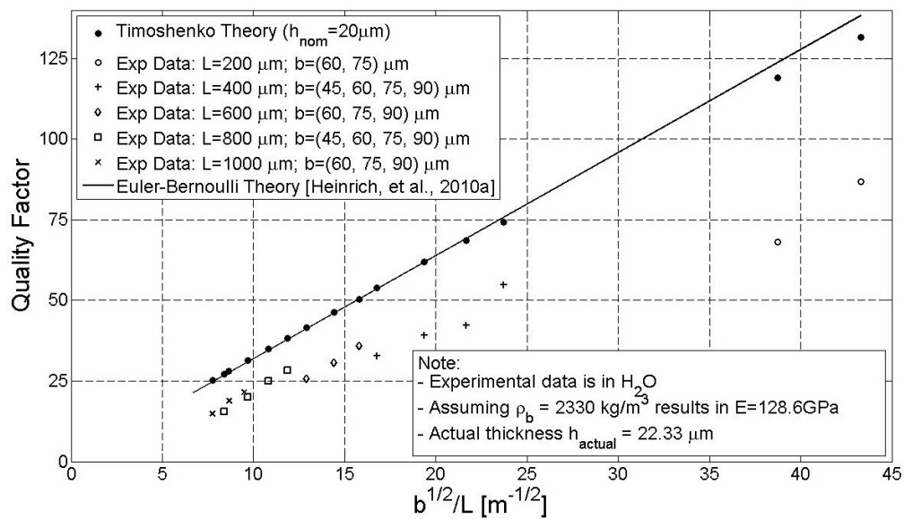
Figure 4-45: Comparison of Current In-Fluid, Timoshenko Model to Experimental [Beardslee et al., 2012] Quality Factor for First Lateral Flexural Mode, Nominal Thickness 20 \mu m Using \sqrt{E / 12\rho_b} = 2.1447 \text{ km/sec} and \sqrt{E / kG} = 2
