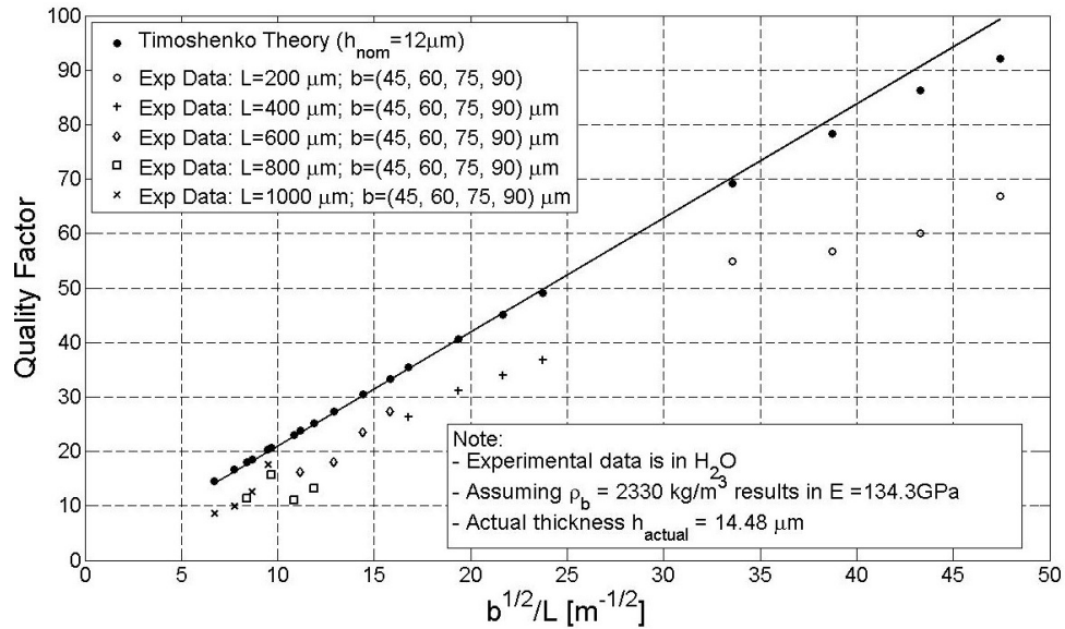
Figure 4-44: Comparison of Current In-Fluid, Timoshenko Model to Experimental [Beardslee et al., 2012] Quality Factor for First Lateral Flexural Mode, Nominal Thickness 12 \mu m Using \sqrt{E / 12\rho_b} = 2.1920 \text{ km/sec} and \sqrt{E / kG} = 2
