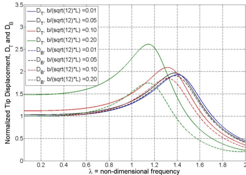
Figure 4-7: Frequency Response Curves of Normalized Tip Displacement of Various Geometries, r = b / (L\sqrt{12}) for \sqrt{E/kG} = 2 and \zeta = 2 Under Harmonic Tip Load Measured by D_T and D_B for the First Mode Response
