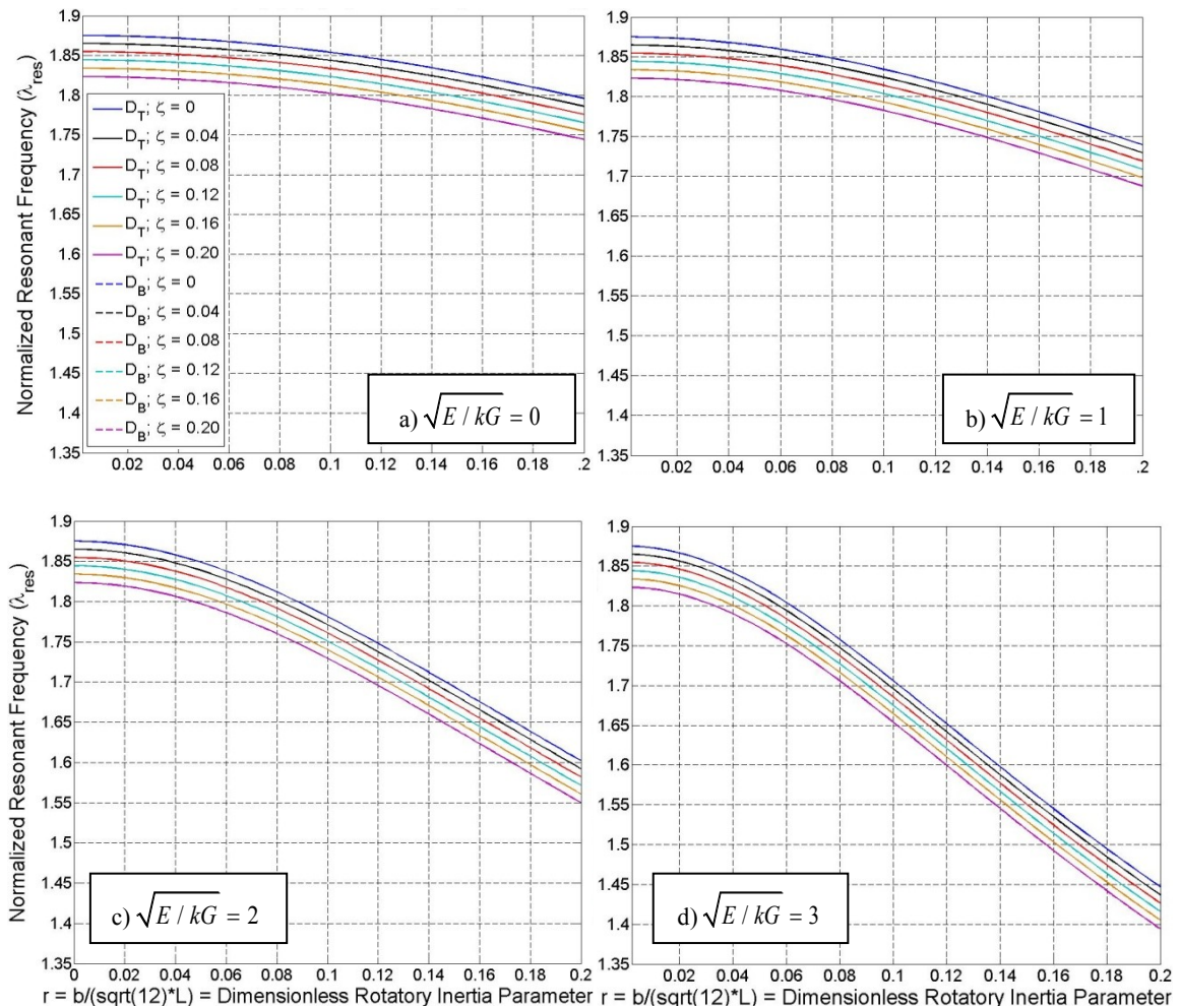
Figure 4-8: Resonant Frequency at Tip ( \zeta=1 ) for Various Fluid Resistance parameters ( \zeta ), for r = b/(L\sqrt{12}) \in [0,0.2] Measured by D_T and D_B : (a) \sqrt{E/kG} = 0 , (b) \sqrt{E/kG} = 1 , (c) \sqrt{E/kG} = 2 , (d) \sqrt{E/kG} = 3
