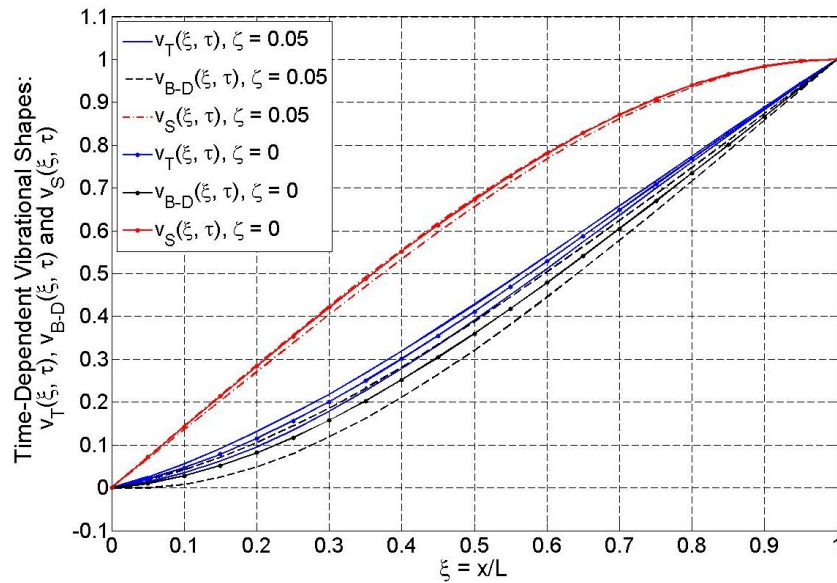
Figure 4-20: Vibrational Shapes v_T(\xi, \tau) , v_{B-D}(\xi, \tau) , and v_S(\xi, \tau) Due to Harmonic Support Rotation for \lambda = 1.6674 , \zeta = 0.05 , b/L = 0.45 ( r = 0.13 ) and \sqrt{E/kG} = 2
