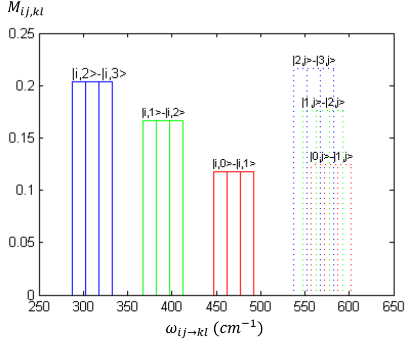
Fig. 4.2 Transition frequency diagram for the gate NOT in the two-qubit system described by (\Delta_1, \Delta_2, \Delta_{12}) = (5, 40, 15) \text{ cm}^{-1} . None of frequencies are in resonance.
