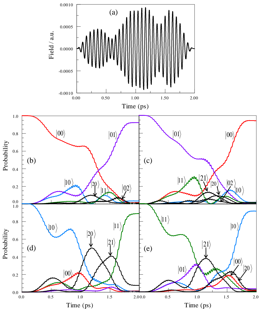
Fig. 5.2 Numerical results for the gate NOT in the two-qubit system described by (\Delta_1, \Delta_2, \Delta_{12}) = (30, 30, 5) \text{ cm}^{-1} . (a) Optimized 2 ps laser pulse; [(b)-(e)] Evolution of the state populations during the pulse for state-to-state transitions given by Eq. (2.2.1).
