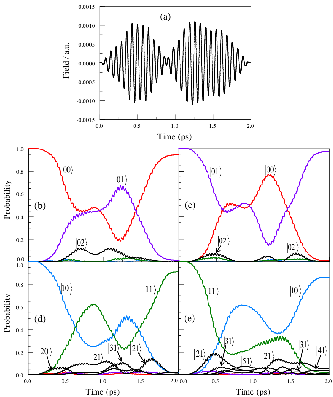
Fig. 5.5 Numerical results for the gate CNOT in the two-qubit system described by (\Delta_1, \Delta_2, \Delta_{12}) = (15, 40, 30) \text{ cm}^{-1} . (a) Optimized 2 ps laser pulse; [(b)-(e)] Evolution of the state populations during the pulse for state-to-state transitions given by Eq. (2.3.1).
