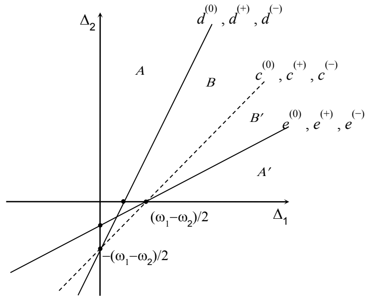
Fig. 6.1 Positions of three triplets of the low fidelity planes as they cross the (\Delta_1, \Delta_2) plane. The triplet planes c^{(0)} , c^{(+)} and c^{(-)} in Fig. 2.4 (b) affect both qubits equally. The triplet planes d^{(0)} , d^{(+)} and d^{(-)} in Fig. 2.4 (c) affect transformations of the second qubit, while the triplet planes e^{(0)} , e^{(+)} and e^{(-)} for Eqs. (6.9) (a, b, c) affect transformations of the first qubit. Letters A and B indicate high fidelity regions when only second (target) qubit is considered (comparing Figs. 4.1 and 4.4). Letters A' and B' indicate similar region for the first (control) qubit. Note that the intersection points are defined by the frequency difference.
