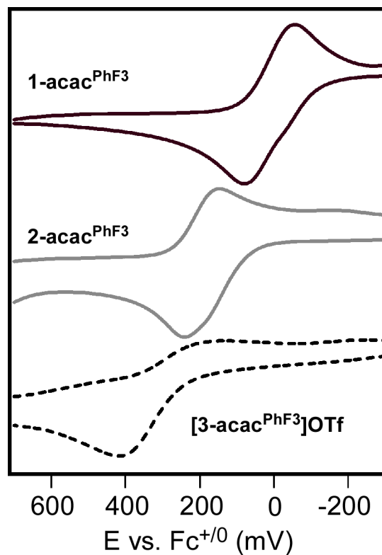
Figure 2.6. Cyclic voltammograms of 1-acac PhF3 , 2-acac PhF3 , and [3-acac PhF3 ]OTf in MeCN (or 1:1 MeCN:CH 2 Cl 2 for 2-acac PhF3 ) with 60 mM (NBu 4 )PF 6 as the supporting electrolyte and a scan rate of 100 mV/s.
