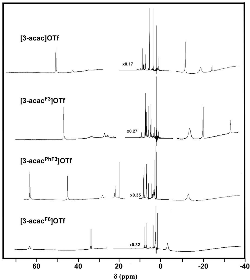
Figure 2.5. ^1\text{H} NMR of complexes 3\text{-acac}^{\text{X}} in \text{MeCN-}d_3 . Note that peak intensities in the middle portions of the spectra were reduced for the sake of clarity.
