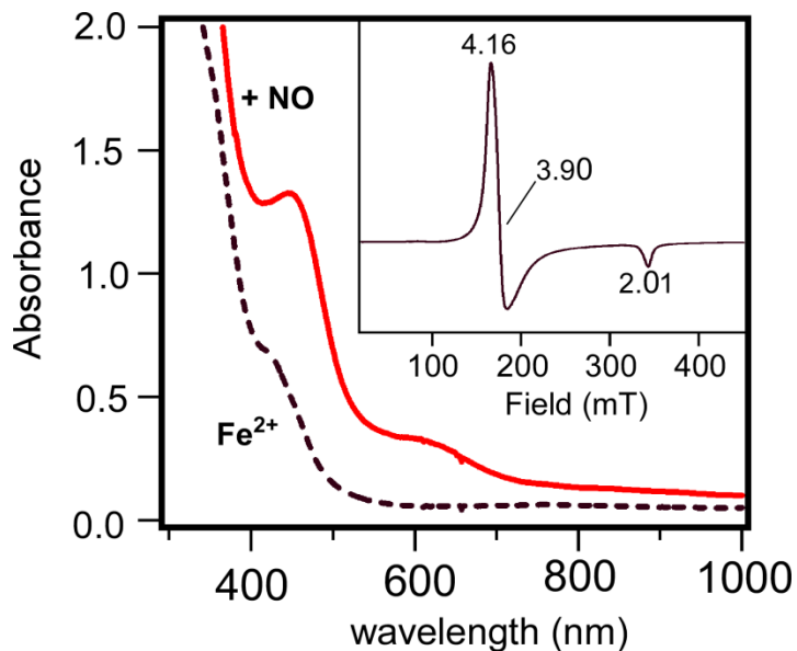
Figure 2.7. Absorption spectra of 3-acac in MeCN at -40\text{ }^{\circ}\text{C} before and after addition of NO. [\text{Fe}] = 2.1\text{ mM} . Inset: X-band EPR spectrum of the Fe-NO adduct of 3-acac in frozen MeCN. Instrumental parameters: frequency = 9.629 GHz; power = 2.0 mW; modulation = 12 G; temperature = 10 K.
