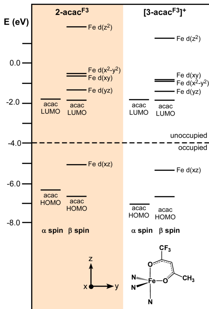
Figure 2.10. MO energy diagrams for geometry-optimized models of 2\text{-acac}^{\text{F}3} and [\mathbf{3}\text{-acac}^{\text{F}3}]^+ obtained from DFT calculations. To account for differences in overall charge, the computed MO energies for [\mathbf{3}\text{-acac}^{\text{F}3}]^+ were uniformly increased by 2.41 eV, such that the acac HOMOs are isoenergetic for the two models (see main text for more details).
