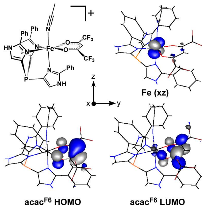
Figure 2.9. Isosurface plots of spin-down MOs computed for [3-acac F6 (MeCN)] + by DFT.
