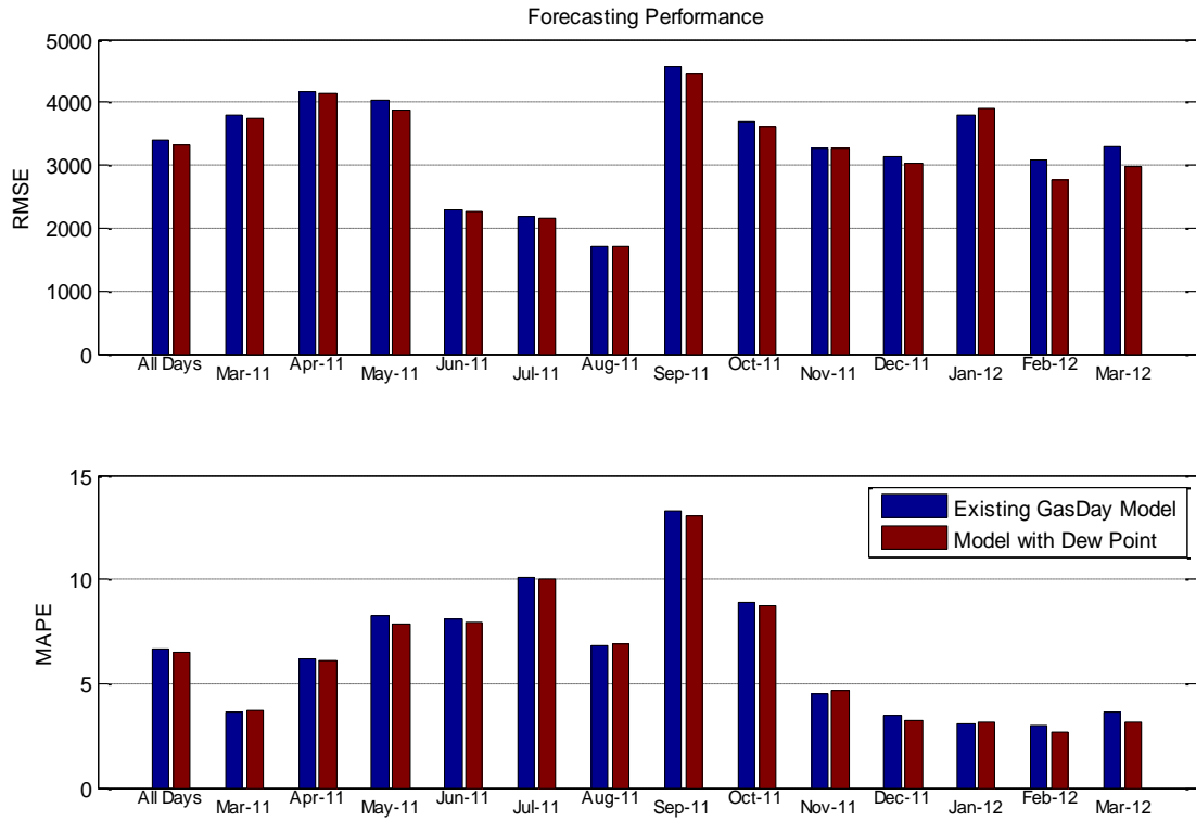
Figure 3.6 Adding Dew Point to the existing GasDay model
