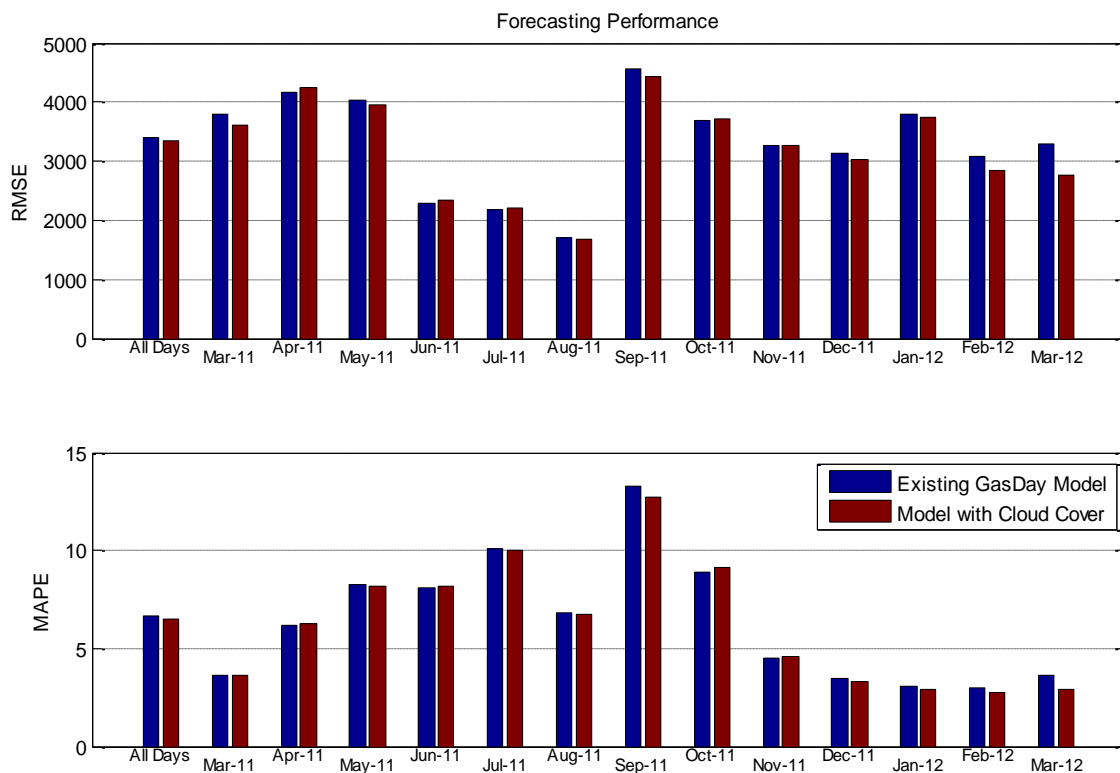
Figure 3.4 Adding Cloud Cover to the existing GasDay model
