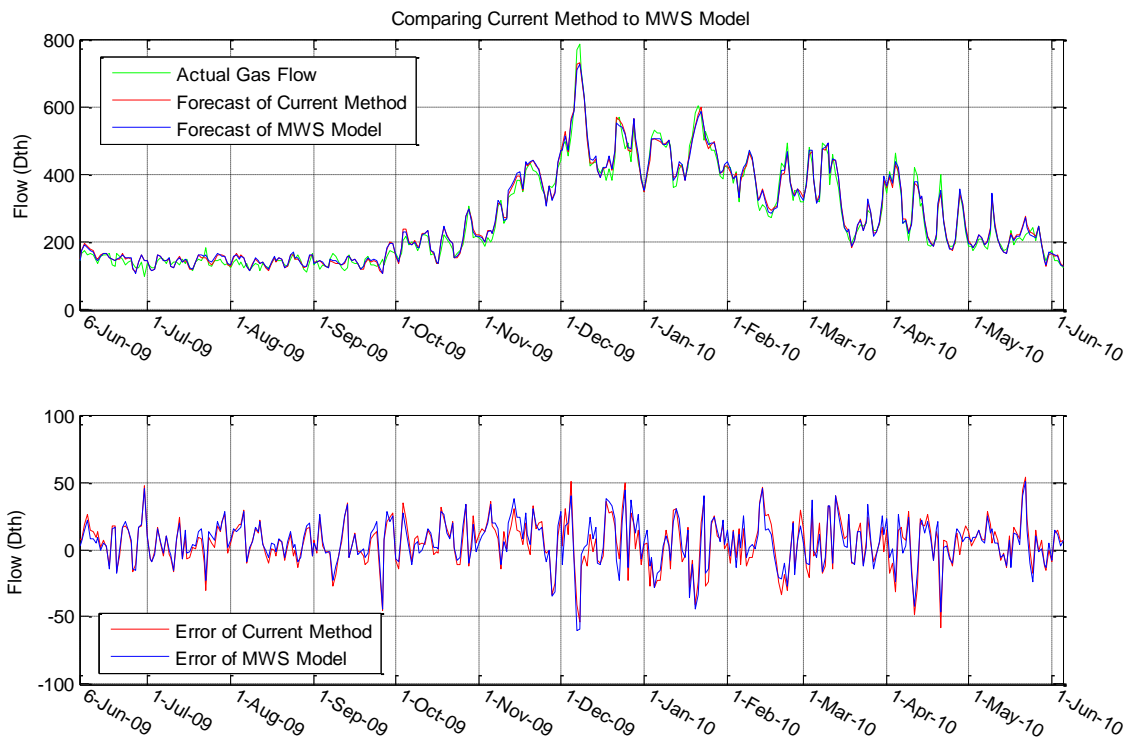
Figure 4.6 Gas demand forecasting for 2010
