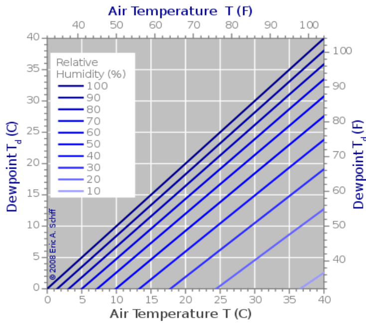
Figure 2.2 Dew Point vs. air temperature at varying relative humidity [49]
