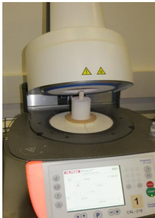
Figure 3. Press furnace Programat EP 5000.
