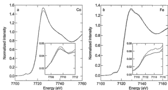
Figure 1 X-ray absorption K-edge spectra for EcMetAP : (a) [Co(II)Co(II)( EcMetAP )] (solid) and [Co(II)]( EcMetAP ) (dotted); (b) [Fe(II)Fe(II)( EcMetAP )] (solid) and [Fe(II)]( EcMetAP ) (dotted). In the inset, the preedge 1s \rightarrow 3d transition is expanded.
