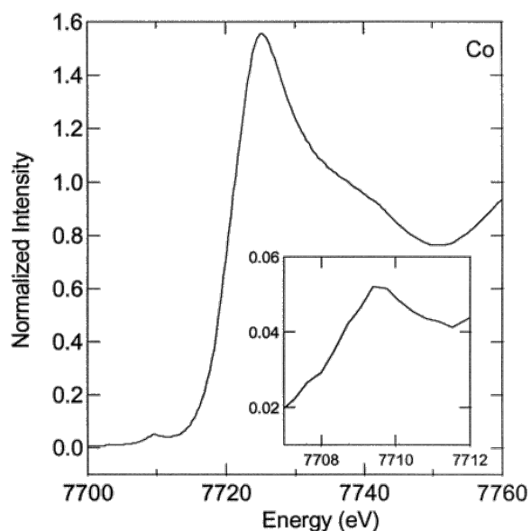
Figure 6 X-ray absorption K-edge spectra for [Co(II)Co(II)(EcMetAP)] plus fumagillin. In the inset, the pre-edge 1s \rightarrow 3d transition is expanded.
