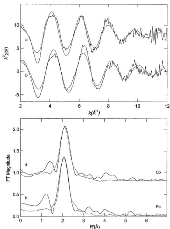
Figure 4 k^3 -weighted EXAFS (top) and Fourier transforms (bottom, over k = 2\text{--}12 \text{\AA}^{-1} ) for (a) [\text{Co(III)Co(III)(EcMetAP)}] (solid) and the calculated spectra for \text{Co-O}_5 (dotted; fit 14, Table 2) and (b) [\text{Fe(III)Fe(III)(EcMetAP)}] and the calculated spectra for \text{Fe-O}_5 (dotted; fit 11, Table 3).
