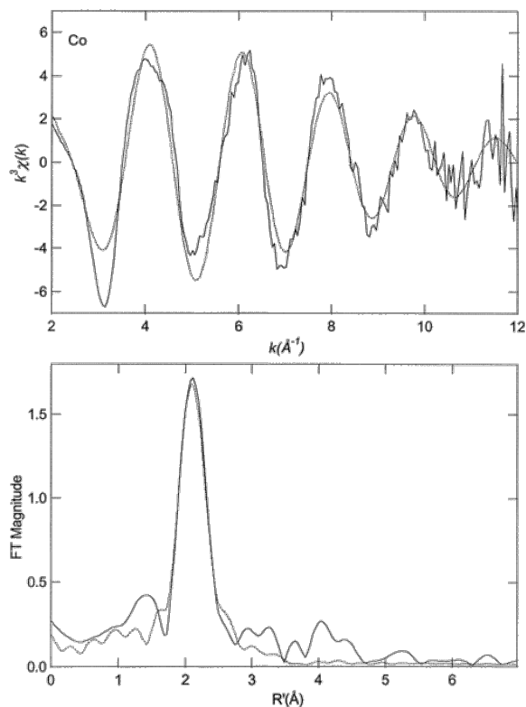
Figure 5 k^3 -weighted Co EXAFS (top) and Fourier transforms (bottom, over k = 2\text{--}12 \text{ \AA}^{-1} ) for [\text{Co(II)Co(II)}(\text{EcMetAP})] plus fumagillin (solid) and the calculated spectra for Co–O 6 (dotted; fit 3, Table 4).
