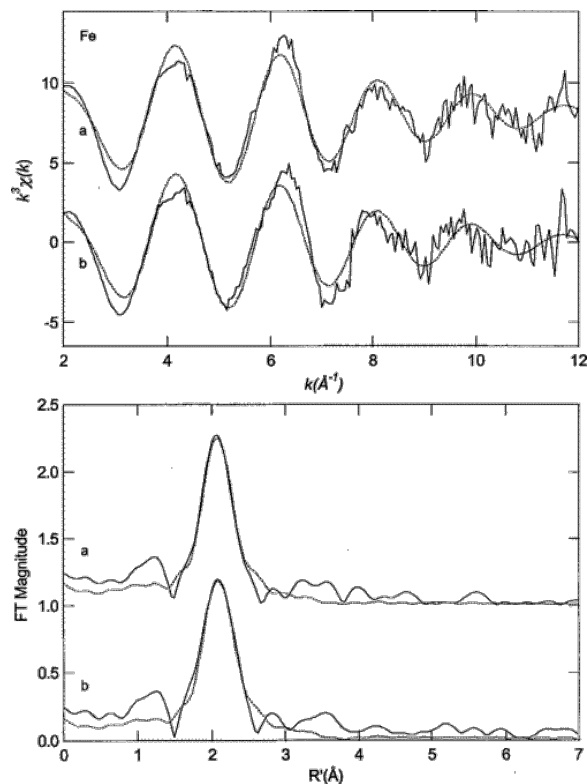
Figure 3 k^3 -weighted Fe EXAFS (top) and Fourier transforms (bottom, over k = 2\text{--}12 \text{ \AA}^{-1} ) for (a) [Fe(II)Fe(II)( EcMetAP )] (solid) and the calculated spectra for Fe–O 5 (dotted; fit 7, Table 3) and (b) [Fe(II)_( EcMetAP )] (solid) and the calculated spectra for Fe–O 5 (dotted; fit 2, Table 3).
