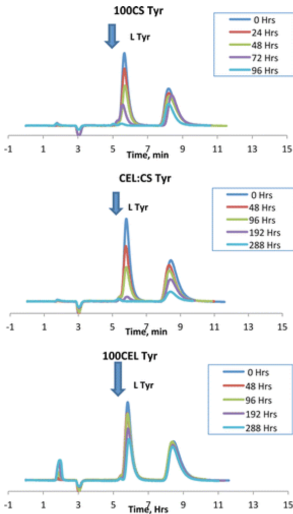
Figure 1. HPLC chromatograms for the sorption of d- and l-Tyr on the different polysaccharide composites.
