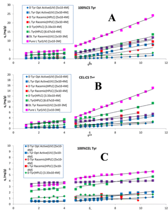
Figure 4. Intraparticle diffusion plots for the sorption of d- and l-Tyr from solutions with different concentrations and/or enantiomeric compositions by (A) 100CS, (B) CEL/CS, and (C) 100CEL composites.
