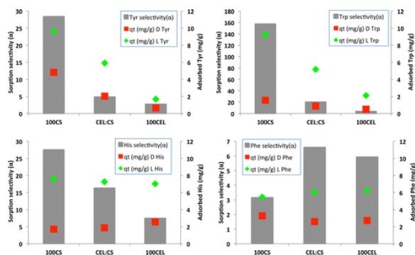
Figure 5. Comparison of the selectivity of the different composite materials with the four amino acids studied. The initial concentration of each racemic amino acid was 1.0 \times 10^{-3} M.
