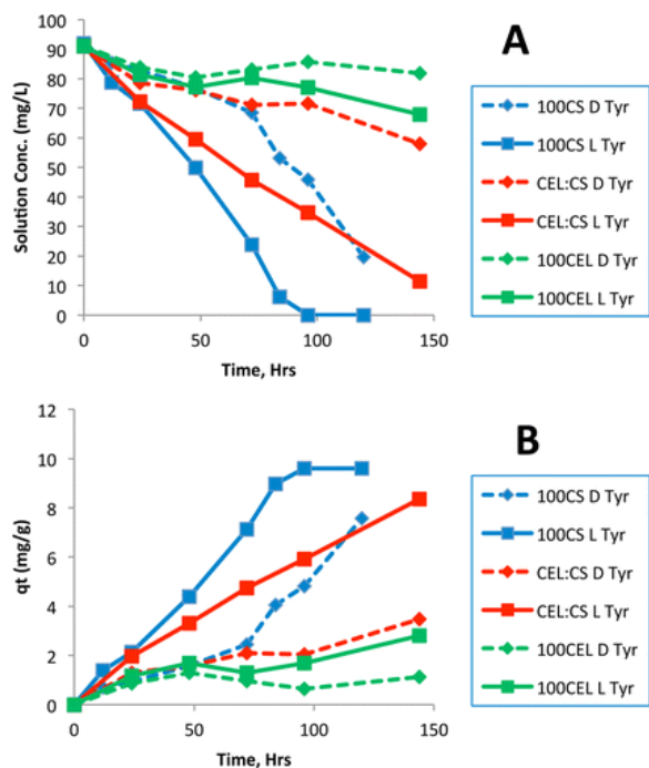
Figure 2. (A) Change in solution concentration with time for a Tyr racemic solution. (B) Adsorption of different Tyr enantiomers by the different composites.
