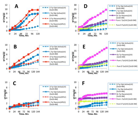
Figure 3. Sorption of d- and l-Tyr enantiomers from different solutions using (A, D) 100% CS, (B, E) the [CEL+CS] composite, and (C, F) the 100CEL composite.
