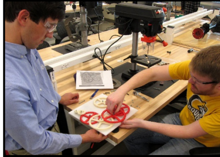
Figure 5: Assembling gear-driven clock mechanisms in Experiment 4.
