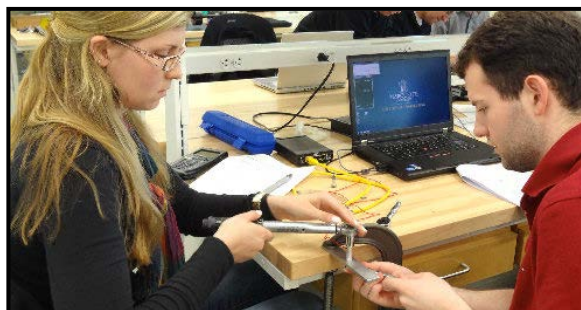
Figure 8: Measuring bolt clamping force in Experiment 7.
